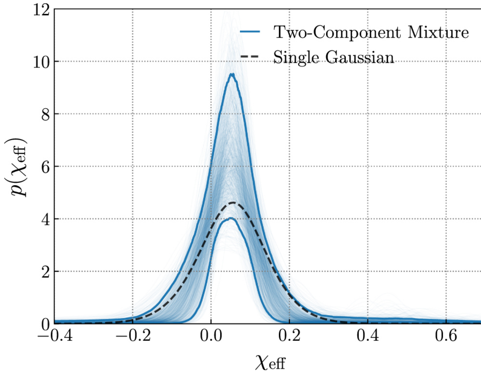
Figure 4. from Thomas A. Callister et al 2022 Astrophys. J. Lett. 937 doi:10.3847/2041-8213/ac847e https://dx.doi.org/10.3847/2041-8213/ac847e © 2022. The Author(s). Published by the American Astronomical Society.
