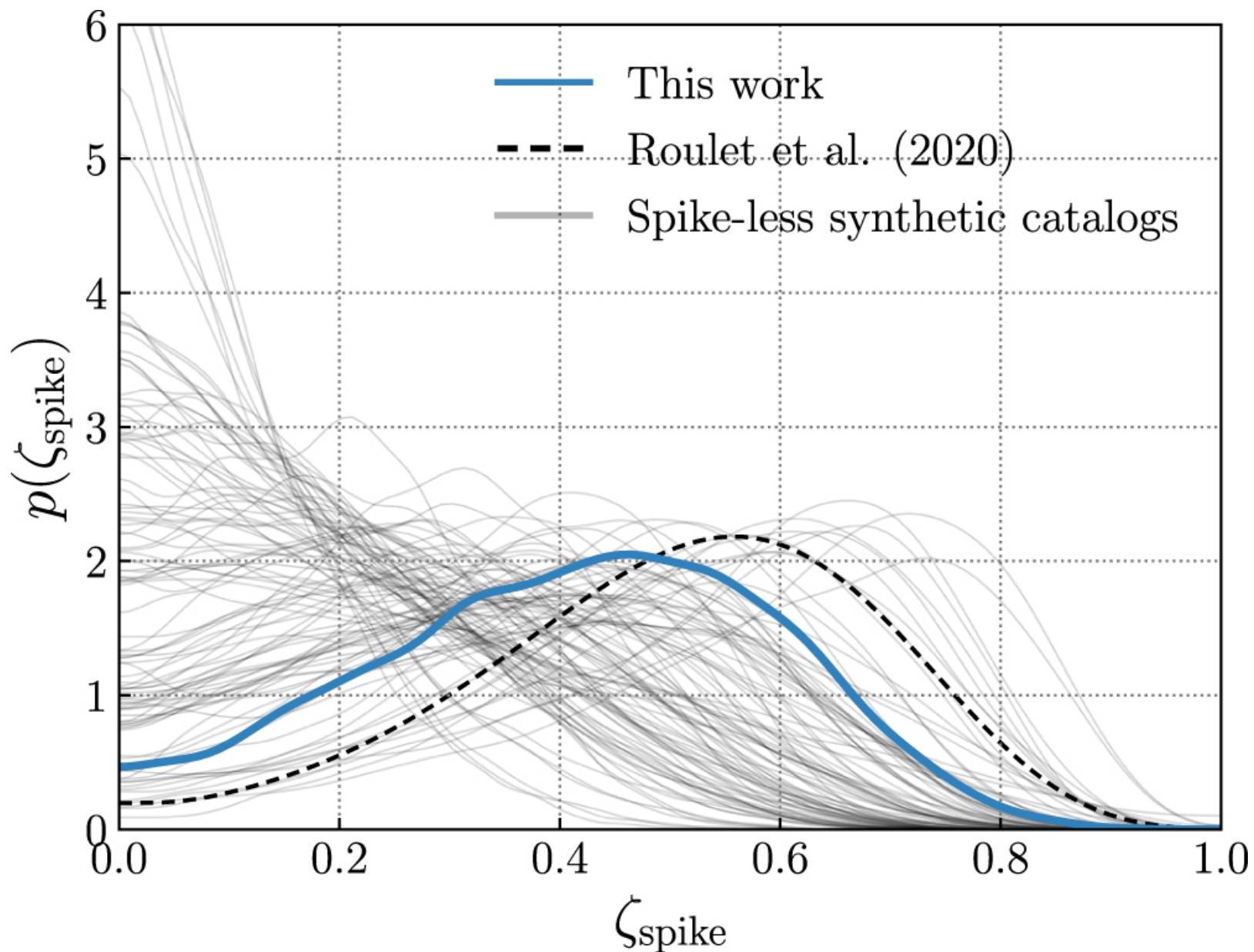
Figure 3. from Thomas A. Callister et al 2022 Astrophys. J. Lett. 937 doi:10.3847/2041-8213/ac847e https://dx.doi.org/10.3847/2041-8213/ac847e © 2022. The Author(s). Published by the American Astronomical Society.
