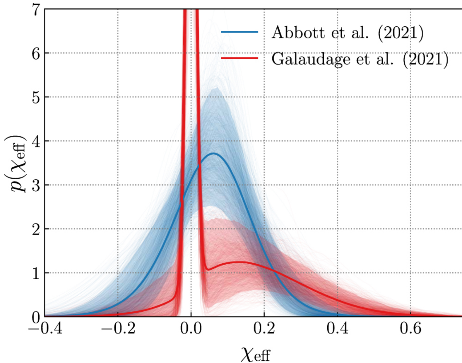
Figure 2. from Thomas A. Callister et al 2022 Astrophys. J. Lett. 937 doi:10.3847/2041-8213/ac847e https://dx.doi.org/10.3847/2041-8213/ac847e © 2022. The Author(s). Published by the American Astronomical Society.
