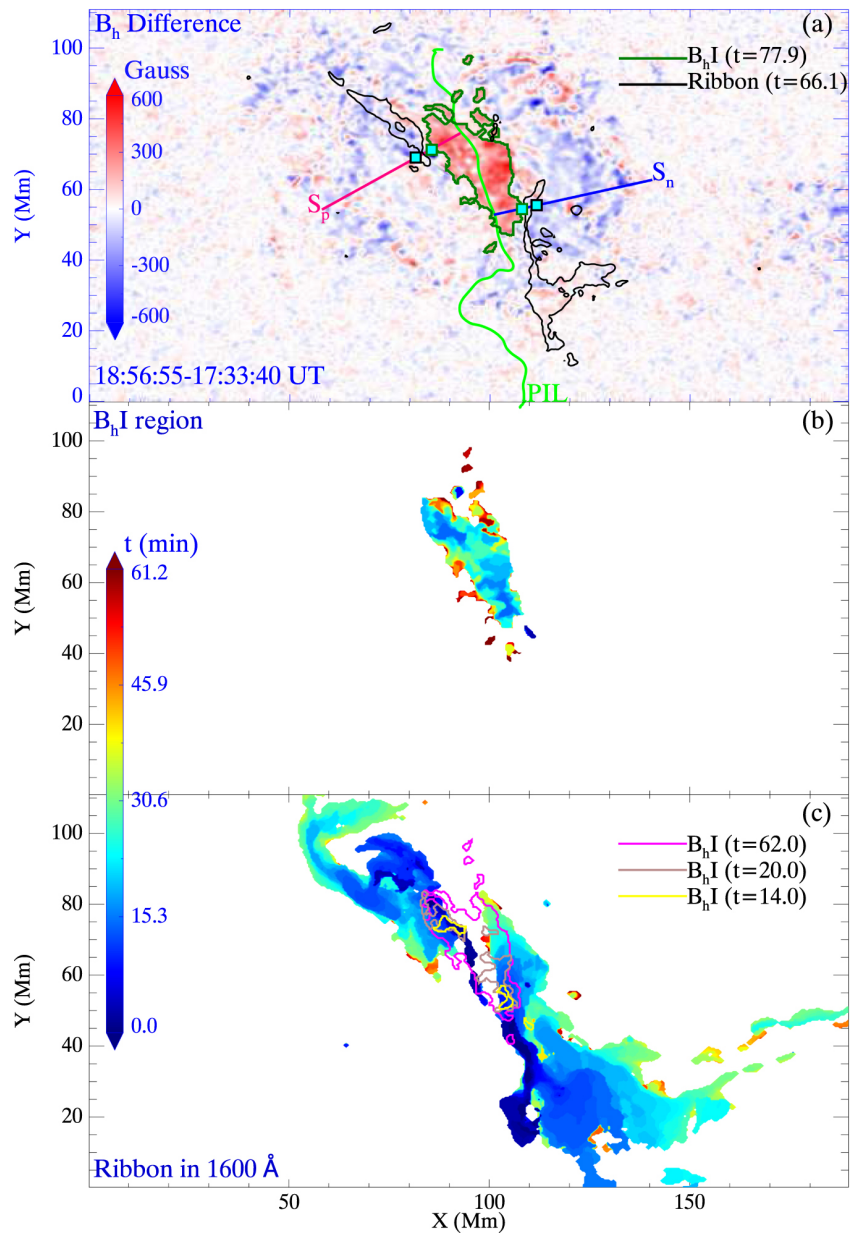
Figure 1. from Lijuan Liu et al 2022 Astrophys. J. Lett. 934 doi:10.3847/2041-8213/ac83bf https://dx.doi.org/10.3847/2041-8213/ac83bf © 2022. The Author(s). Published by the American Astronomical Society.
