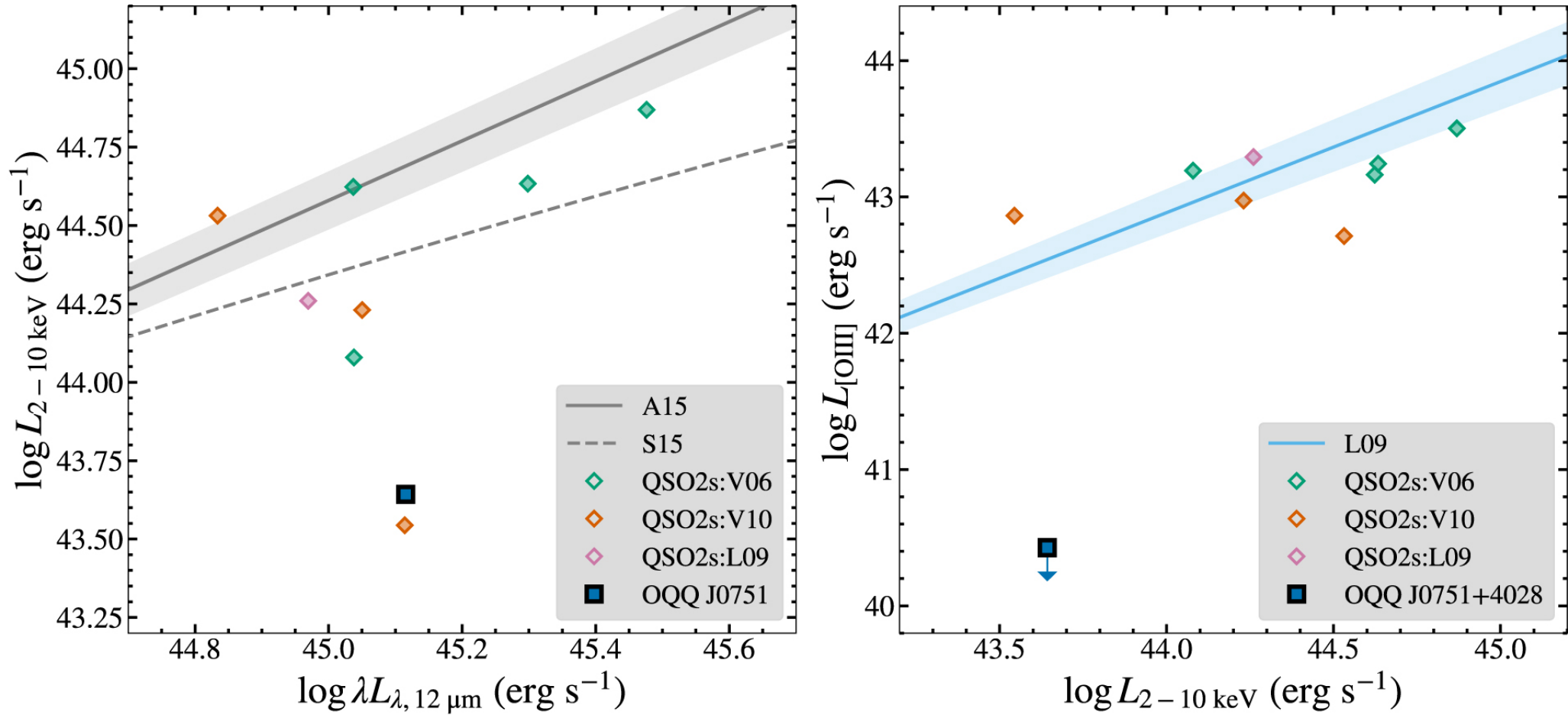
Figure 4. from Claire Greenwell et al 2022 Astrophys. J. Lett. 934 doi:10.3847/2041-8213/ac83a0 https://dx.doi.org/10.3847/2041-8213/ac83a0 © 2022. The Author(s). Published by the American Astronomical Society.
