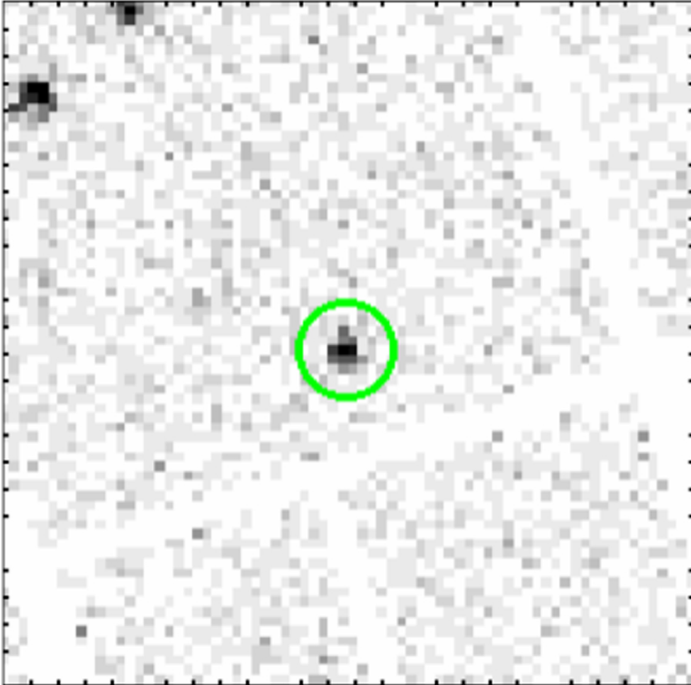
Figure 1. from Claire Greenwell et al 2022 Astrophys. J. Lett. 934 doi:10.3847/2041-8213/ac83a0 https://dx.doi.org/10.3847/2041-8213/ac83a0 © 2022. The Author(s). Published by the American Astronomical Society.
