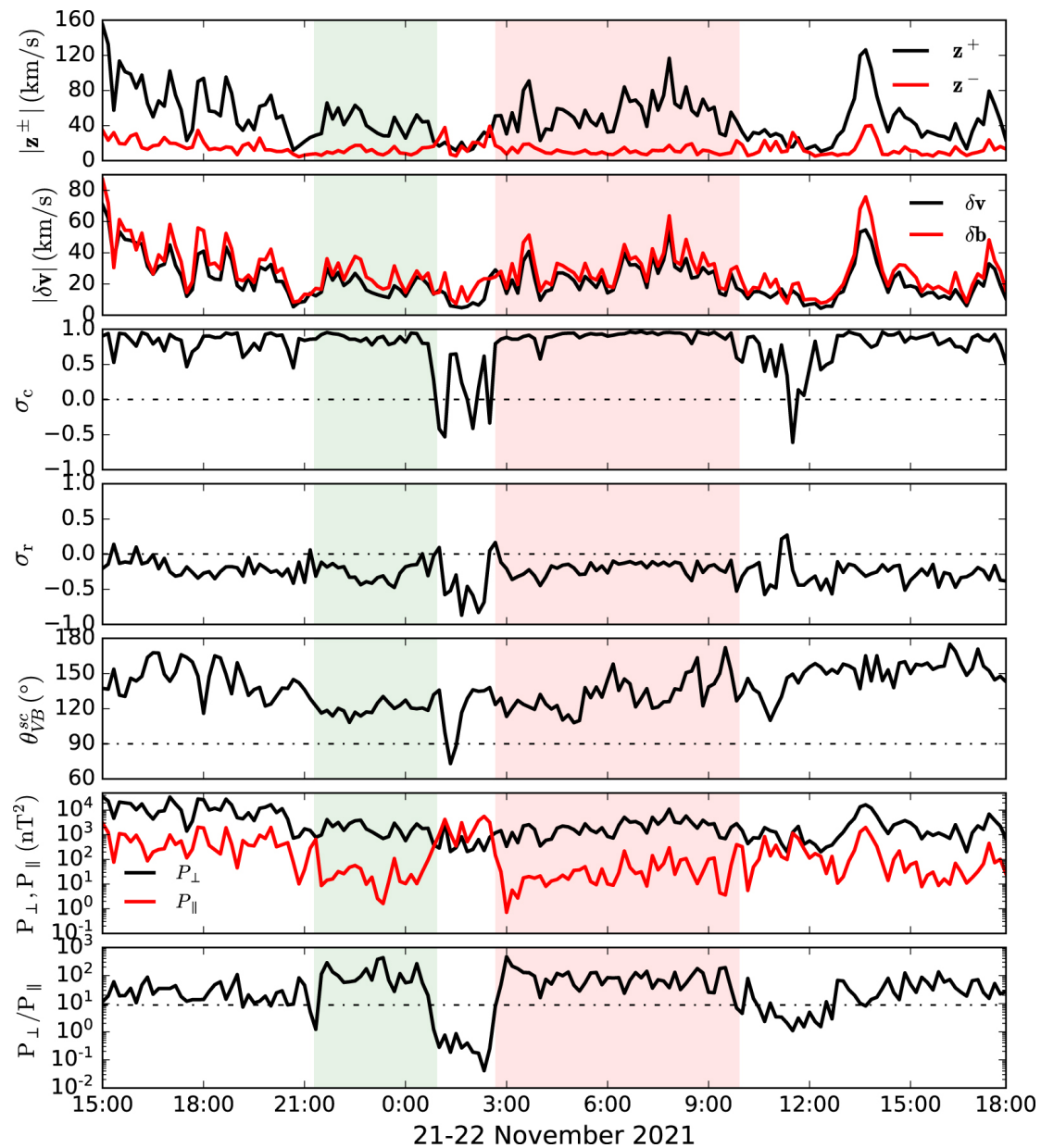
Figure 2. from L.-L. Zhao et al 2022 Astrophys. J. Lett. 934 doi:10.3847/2041-8213/ac8353 https://dx.doi.org/10.3847/2041-8213/ac8353 © 2022. The Author(s). Published by the American Astronomical Society.
