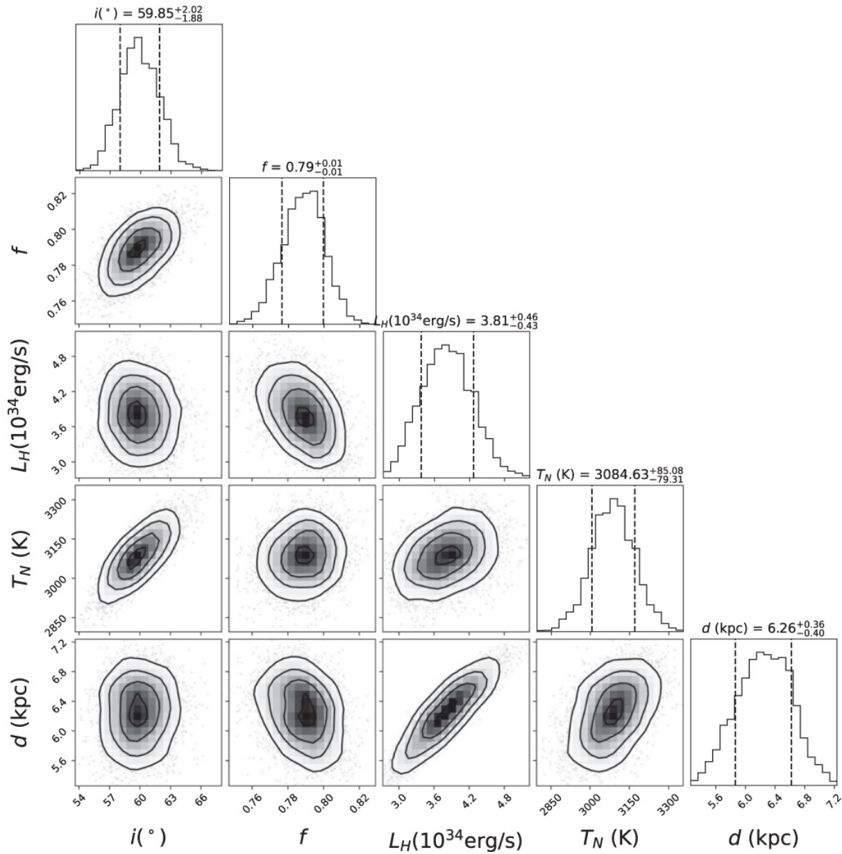
Figure 4. from Roger W. Romani et al 2022 Astrophys. J. Lett. 934 doi:10.3847/2041-8213/ac8007 https://dx.doi.org/10.3847/2041-8213/ac8007 © 2022. The Author(s). Published by the American Astronomical Society.
