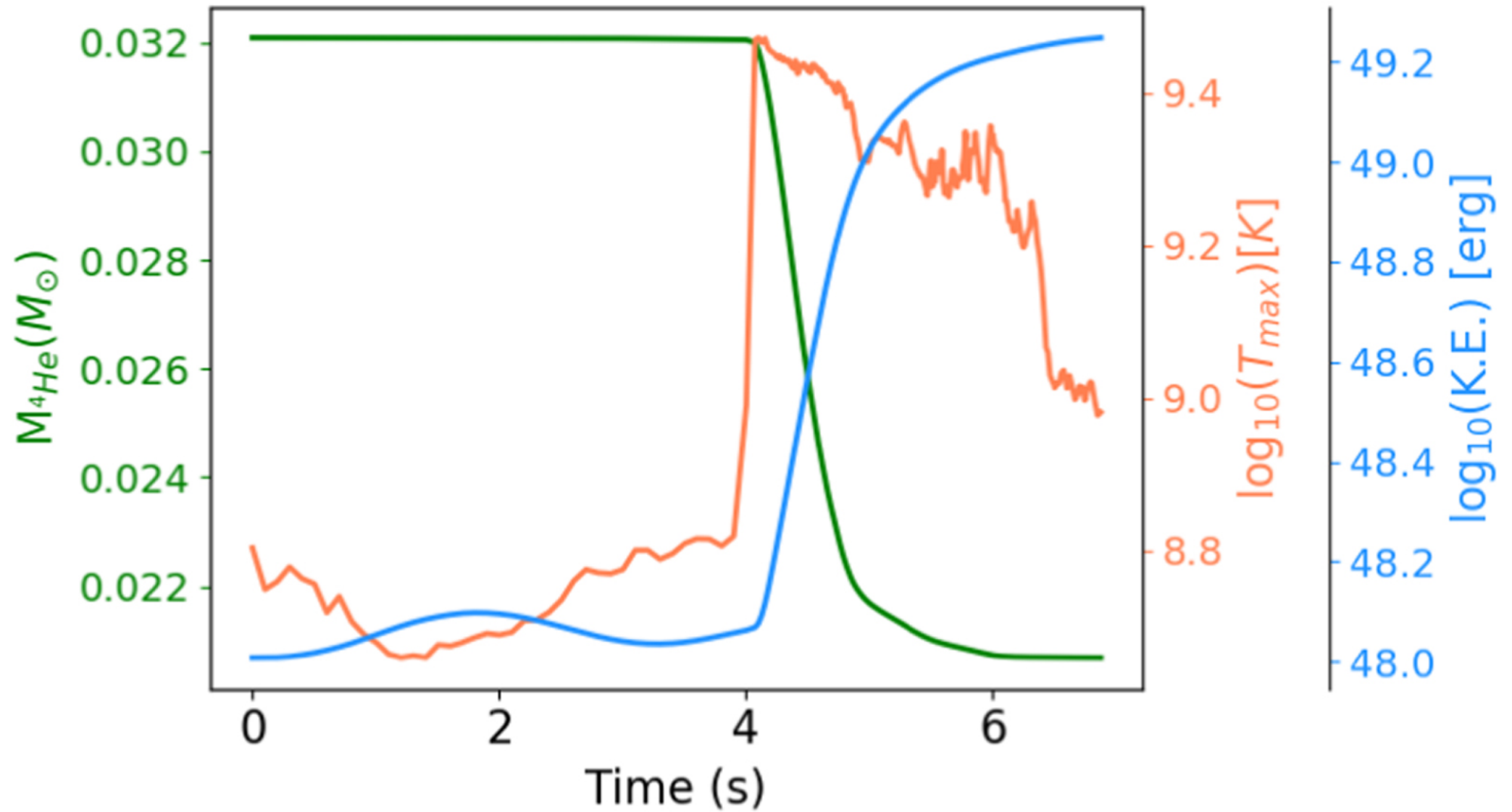
Figure 3. from Niranjan C. Roy et al 2022 Astrophys. J. Lett. 932 doi:10.3847/2041-8213/ac75e7 https://dx.doi.org/10.3847/2041-8213/ac75e7 © 2022. The Author(s). Published by the American Astronomical Society.
