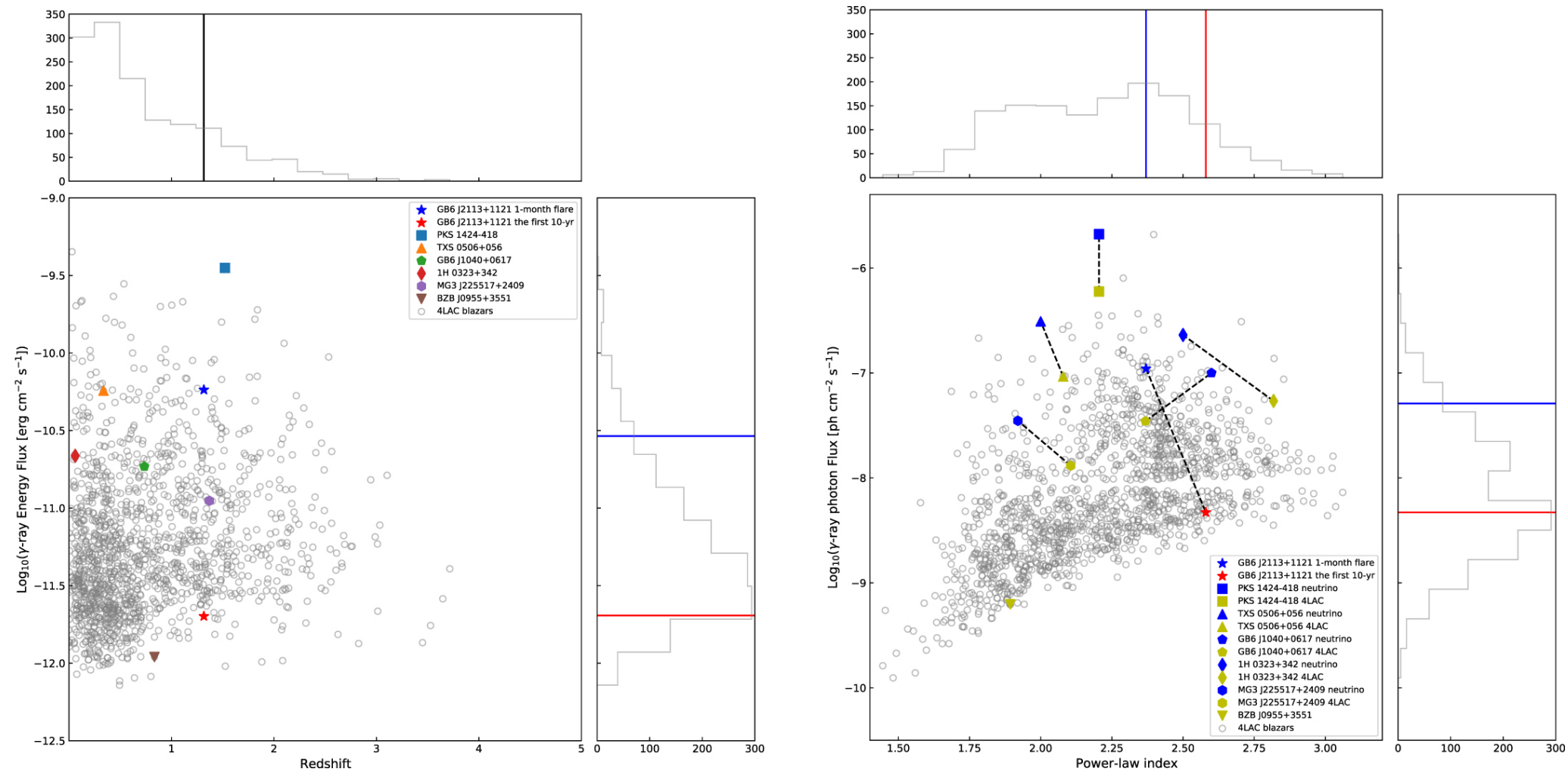
Figure 5. from Neng-Hui Liao et al 2022 Astrophys. J. Lett. 932 doi:10.3847/2041-8213/ac756f https://dx.doi.org/10.3847/2041-8213/ac756f © 2022. The Author(s). Published by the American Astronomical Society.
