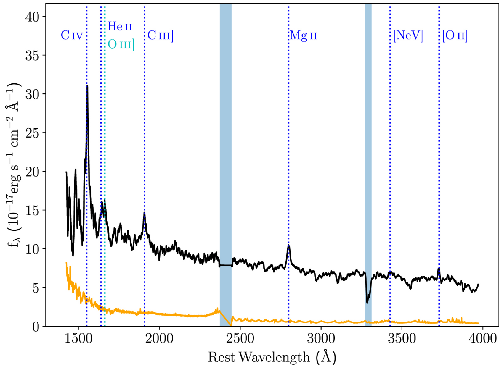
Figure 3. from Neng-Hui Liao et al 2022 Astrophys. J. Lett. 932 doi:10.3847/2041-8213/ac756f https://dx.doi.org/10.3847/2041-8213/ac756f © 2022. The Author(s). Published by the American Astronomical Society.
