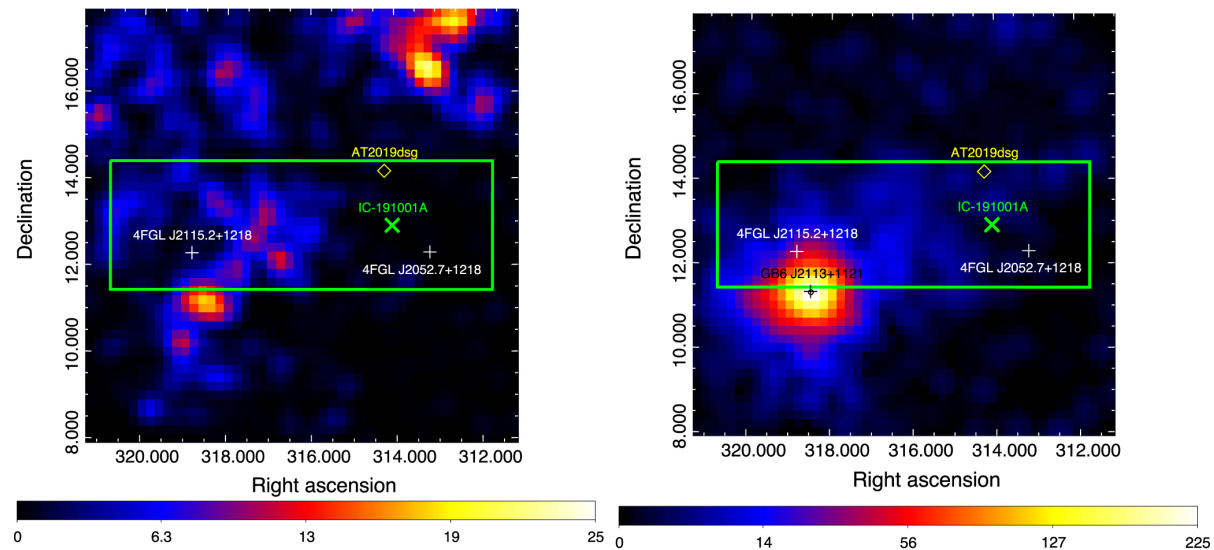
Figure 1. from Neng-Hui Liao et al 2022 Astrophys. J. Lett. 932 doi:10.3847/2041-8213/ac756f https://dx.doi.org/10.3847/2041-8213/ac756f © 2022. The Author(s). Published by the American Astronomical Society.
