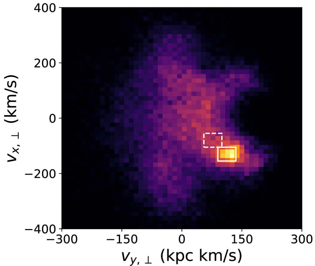
Figure 5. from Thomas Donlon II et al 2022 Astrophys. J. Lett. 932 doi:10.3847/2041-8213/ac7531 https://dx.doi.org/10.3847/2041-8213/ac7531 © 2022. The Author(s). Published by the American Astronomical Society.
