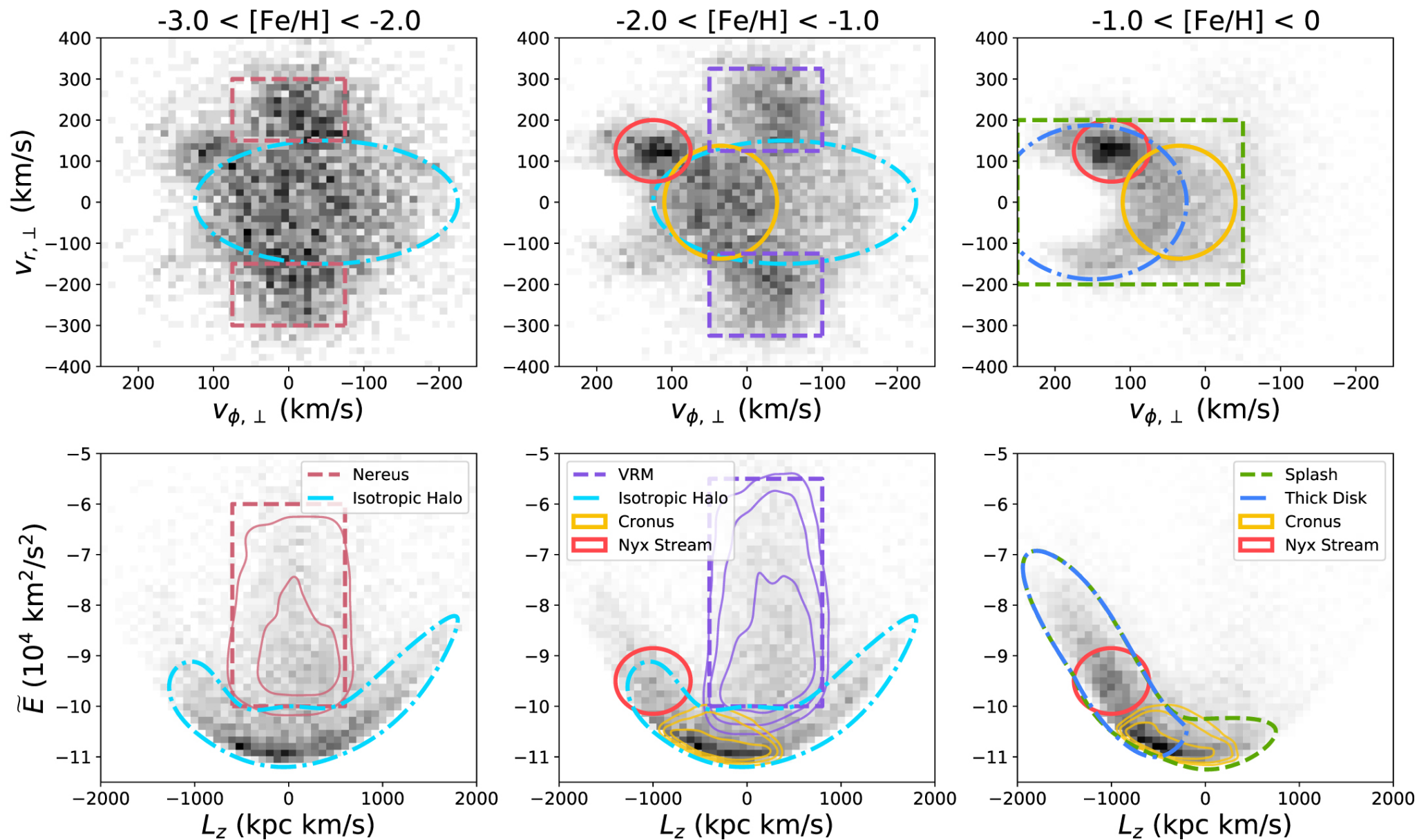
Figure 2. from Thomas Donlon II et al 2022 Astrophys. J. Lett. 932 doi:10.3847/2041-8213/ac7531 https://dx.doi.org/10.3847/2041-8213/ac7531
