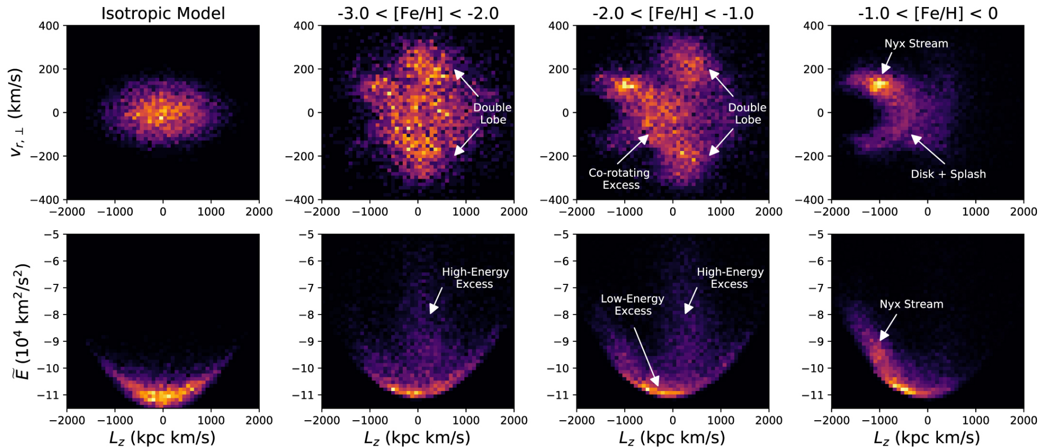
Figure 1. from Thomas Donlon II et al 2022 Astrophys. J. Lett. 932 doi:10.3847/2041-8213/ac7531 https://dx.doi.org/10.3847/2041-8213/ac7531
