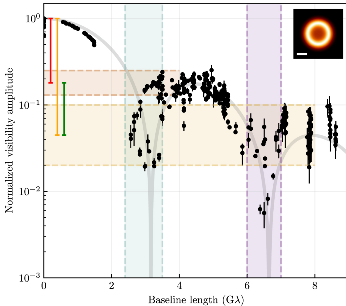
Figure 7. from Event Horizon Telescope Collaboration et al 2022 Astrophys. J. Lett. 930 doi:10.3847/2041-8213/ac6736 https://dx.doi.org/10.3847/2041-8213/ac6736 © 2022. The Author(s). Published by the American Astronomical Society.
