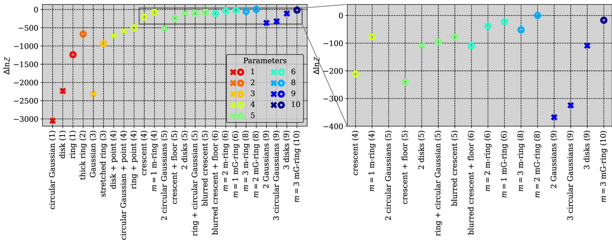
Figure 6. from Event Horizon Telescope Collaboration et al 2022 Astrophys. J. Lett. 930 doi:10.3847/2041-8213/ac6736 https://dx.doi.org/10.3847/2041-8213/ac6736 © 2022. The Author(s). Published by the American Astronomical Society.
