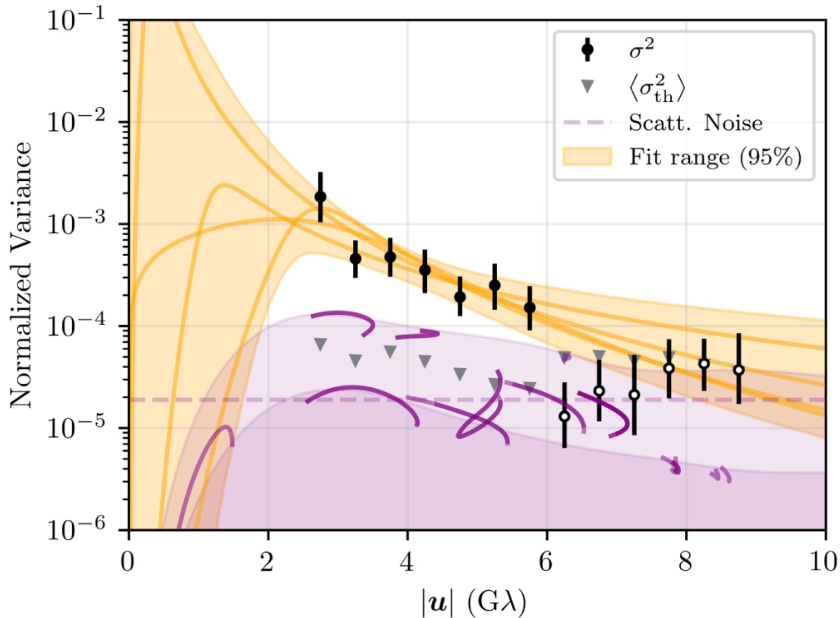
Figure 4. from Event Horizon Telescope Collaboration et al 2022 Astrophys. J. Lett. 930 doi:10.3847/2041-8213/ac6736 https://dx.doi.org/10.3847/2041-8213/ac6736 © 2022. The Author(s). Published by the American Astronomical Society.
