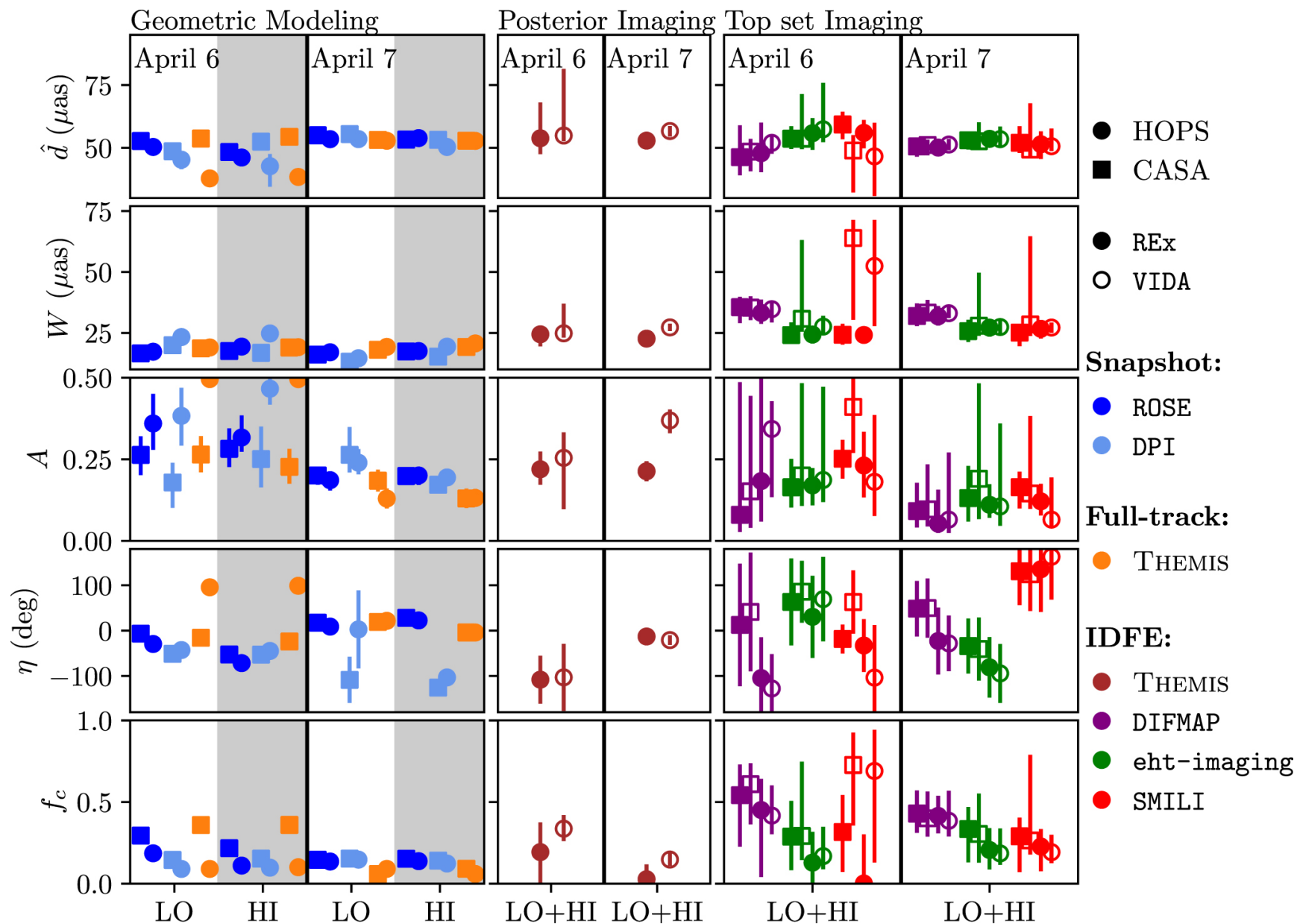
Figure 30. from Event Horizon Telescope Collaboration et al 2022 Astrophys. J. Lett. 930 doi:10.3847/2041-8213/ac6736 https://dx.doi.org/10.3847/2041-8213/ac6736 © 2022. The Author(s). Published by the American Astronomical Society.
