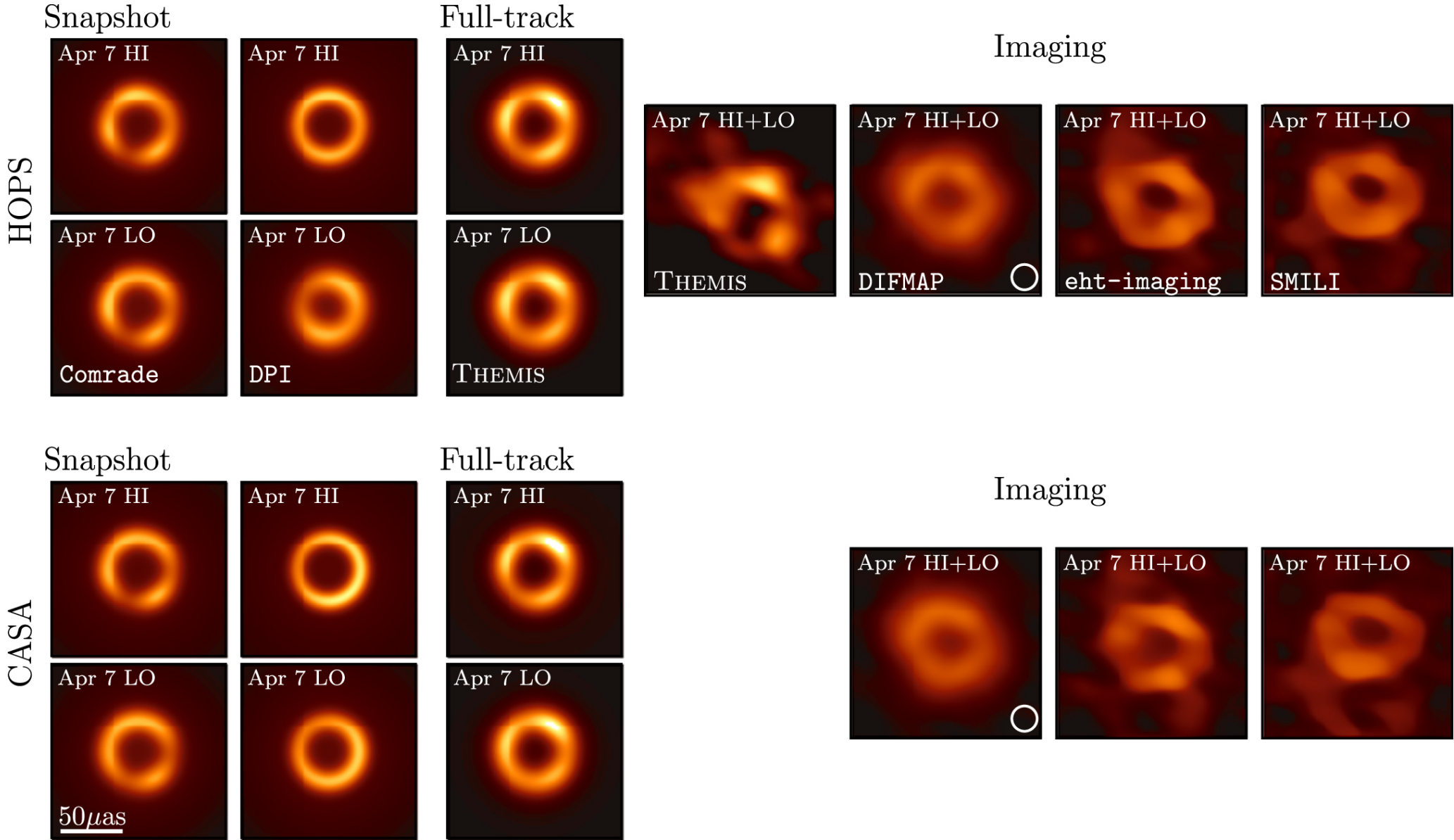
Figure 29. from Event Horizon Telescope Collaboration et al 2022 Astrophys. J. Lett. 930 doi:10.3847/2041-8213/ac6736 https://dx.doi.org/10.3847/2041-8213/ac6736 © 2022. The Author(s). Published by the American Astronomical Society.
