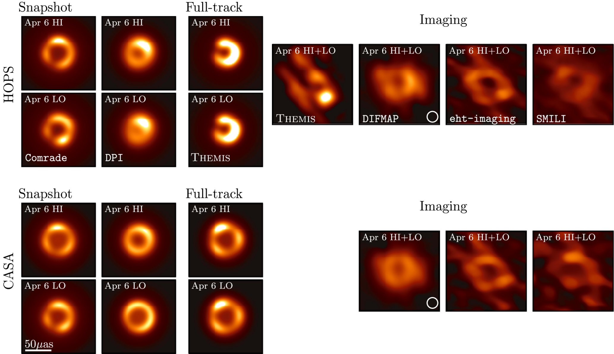
Figure 28. from Event Horizon Telescope Collaboration et al 2022 Astrophys. J. Lett. 930 doi:10.3847/2041-8213/ac6736 https://dx.doi.org/10.3847/2041-8213/ac6736 © 2022. The Author(s). Published by the American Astronomical Society.
