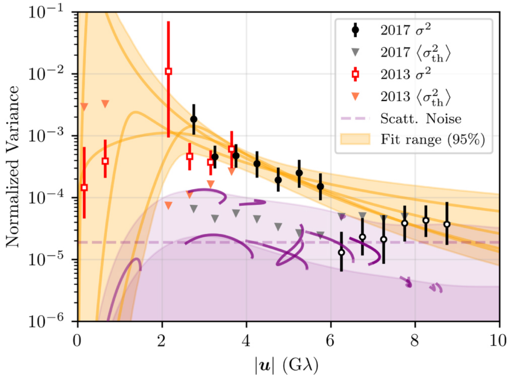
Figure 23. from Event Horizon Telescope Collaboration et al 2022 Astrophys. J. Lett. 930 doi:10.3847/2041-8213/ac6736 https://dx.doi.org/10.3847/2041-8213/ac6736 © 2022. The Author(s). Published by the American Astronomical Society.
