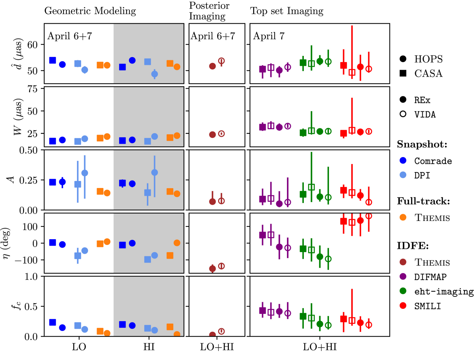
Figure 21. from Event Horizon Telescope Collaboration et al 2022 Astrophys. J. Lett. 930 doi:10.3847/2041-8213/ac6736 https://dx.doi.org/10.3847/2041-8213/ac6736 © 2022. The Author(s). Published by the American Astronomical Society.
