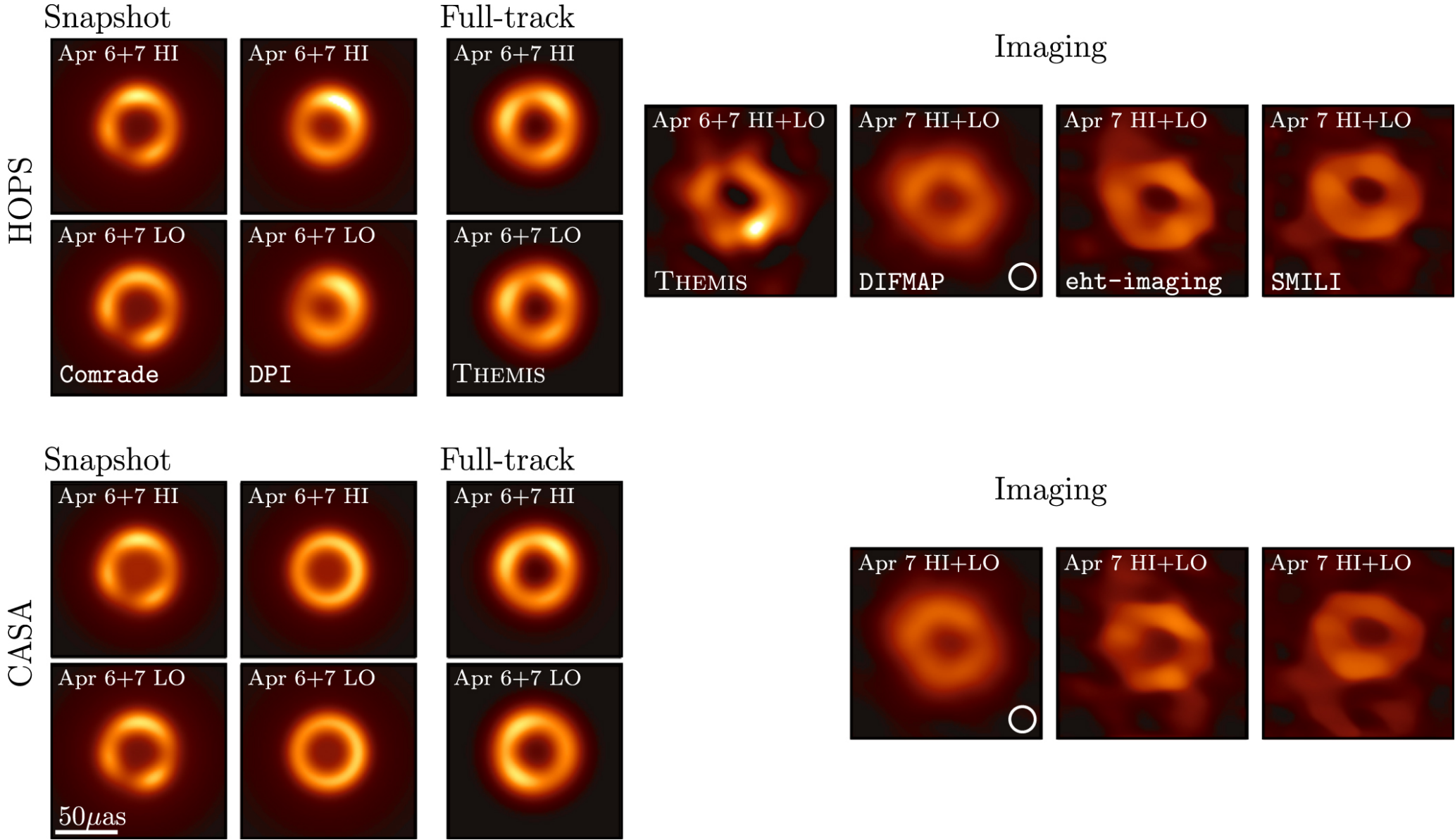
Figure 20. from Event Horizon Telescope Collaboration et al 2022 Astrophys. J. Lett. 930 doi:10.3847/2041-8213/ac6736 https://dx.doi.org/10.3847/2041-8213/ac6736 © 2022. The Author(s). Published by the American Astronomical Society.
