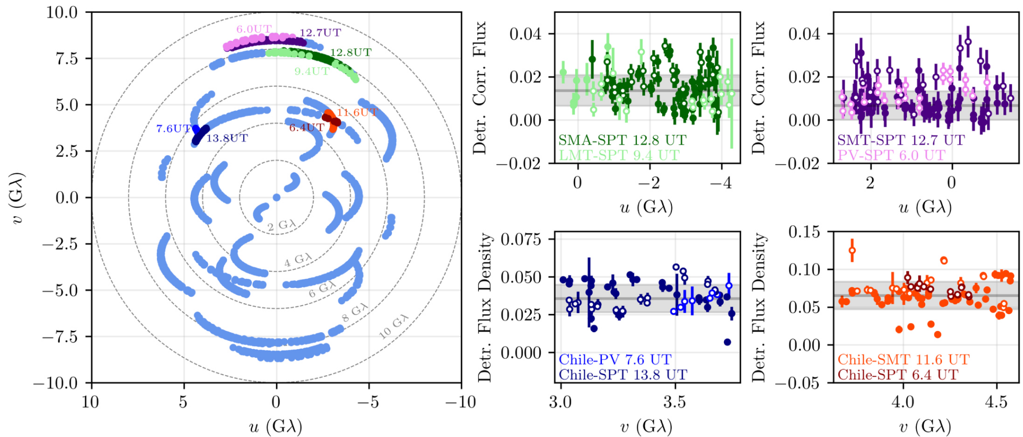
Figure 2. from Event Horizon Telescope Collaboration et al 2022 Astrophys. J. Lett. 930 doi:10.3847/2041-8213/ac6736 https://dx.doi.org/10.3847/2041-8213/ac6736 © 2022. The Author(s). Published by the American Astronomical Society.
