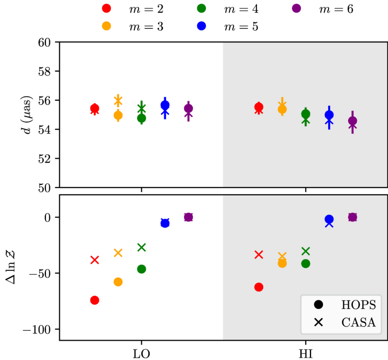
Figure 16. from Event Horizon Telescope Collaboration et al 2022 Astrophys. J. Lett. 930 doi:10.3847/2041-8213/ac6736 https://dx.doi.org/10.3847/2041-8213/ac6736 © 2022. The Author(s). Published by the American Astronomical Society.
