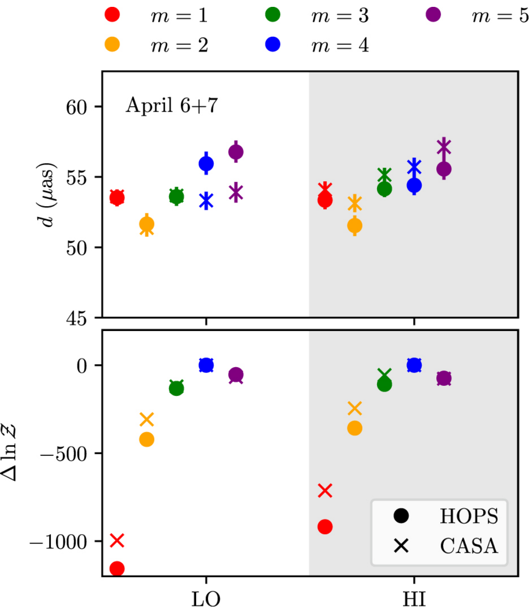
Figure 14. from Event Horizon Telescope Collaboration et al 2022 Astrophys. J. Lett. 930 doi:10.3847/2041-8213/ac6736 https://dx.doi.org/10.3847/2041-8213/ac6736 © 2022. The Author(s). Published by the American Astronomical Society.
