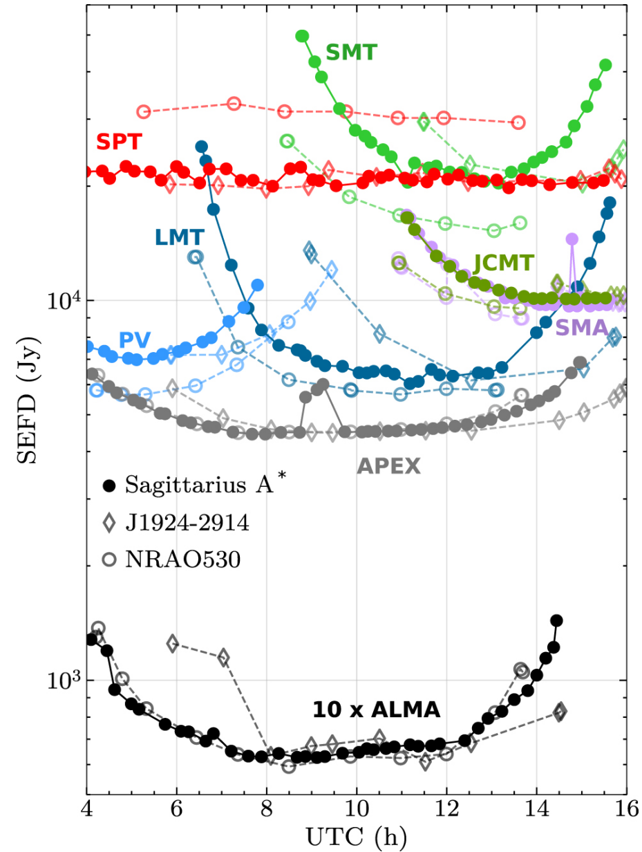
Figure 3. from Event Horizon Telescope Collaboration et al 2022 Astrophys. J. Lett. 930 doi:10.3847/2041-8213/ac6675 https://dx.doi.org/10.3847/2041-8213/ac6675 © 2022. The Author(s). Published by the American Astronomical Society.
