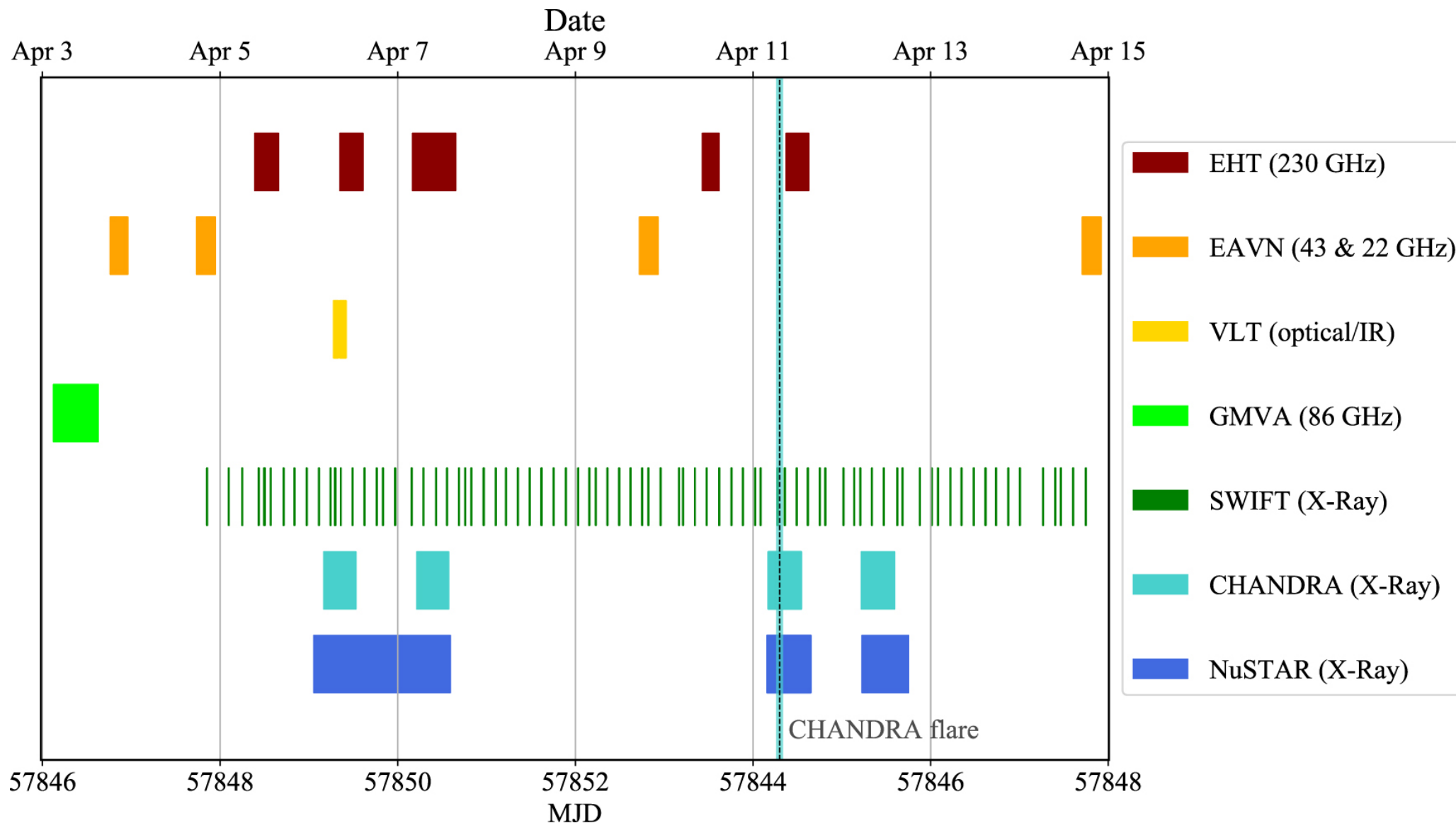
Figure 2. from Event Horizon Telescope Collaboration et al 2022 Astrophys. J. Lett. 930 doi:10.3847/2041-8213/ac6675 https://dx.doi.org/10.3847/2041-8213/ac6675 © 2022. The Author(s). Published by the American Astronomical Society.
