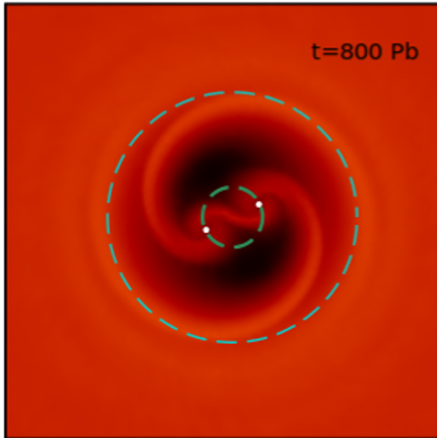
Figure 3. from Alessia Franchini et al 2022 Astrophys. J. Lett. 929 doi:10.3847/2041-8213/ac63a2 https://dx.doi.org/10.3847/2041-8213/ac63a2 © 2022. The Author(s). Published by the American Astronomical Society.
