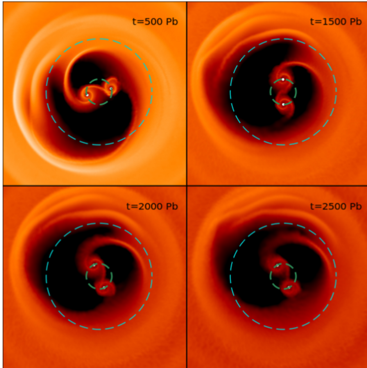
Figure 1. from Alessia Franchini et al 2022 Astrophys. J. Lett. 929 doi:10.3847/2041-8213/ac63a2 https://dx.doi.org/10.3847/2041-8213/ac63a2 © 2022. The Author(s). Published by the American Astronomical Society.
