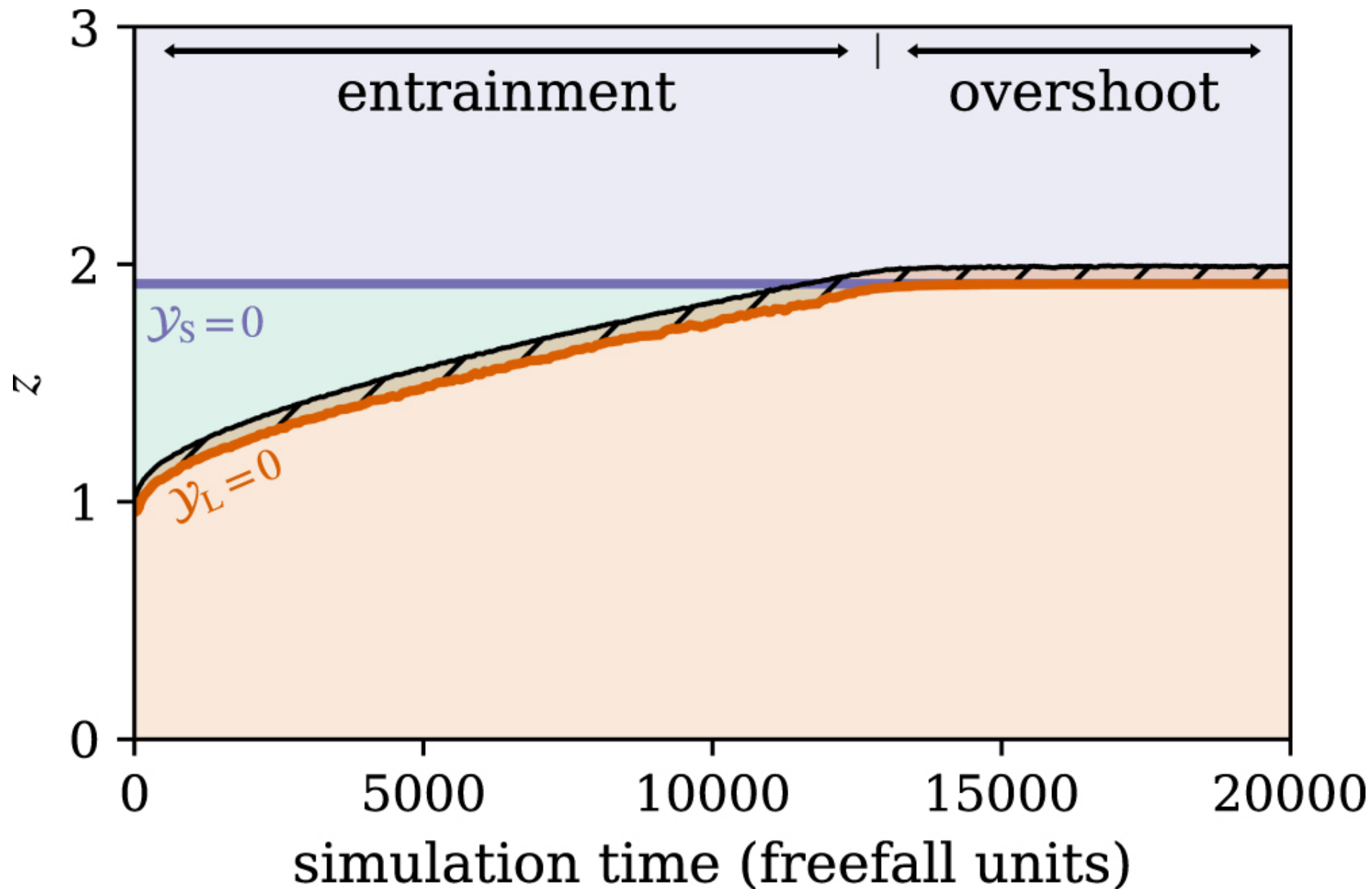
Figure 3. from Evan H. Anders et al 2022 Astrophys. J. Lett. 928 doi:10.3847/2041-8213/ac5cb5 https://dx.doi.org/10.3847/2041-8213/ac5cb5 © 2022. The Author(s). Published by the American Astronomical Society.
