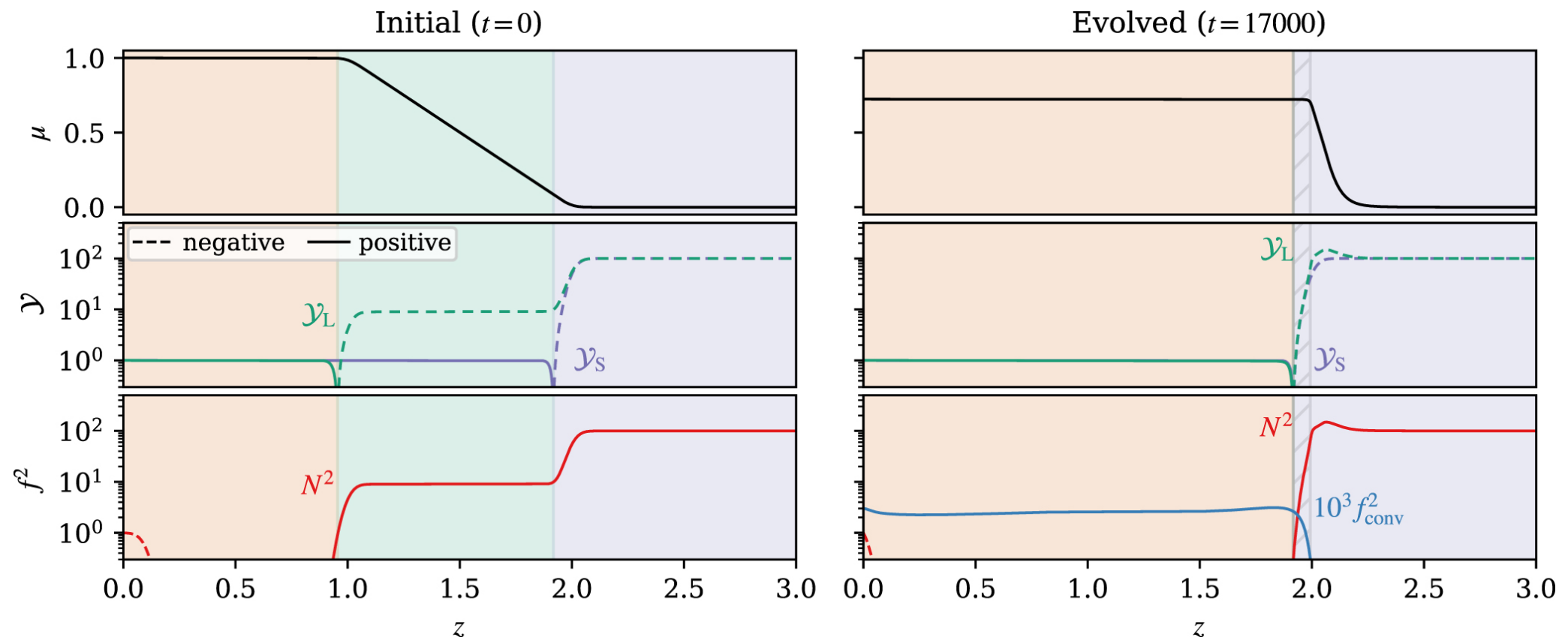
Figure 2. from Evan H. Anders et al 2022 Astrophys. J. Lett. 928 doi:10.3847/2041-8213/ac5cb5 https://dx.doi.org/10.3847/2041-8213/ac5cb5 © 2022. The Author(s). Published by the American Astronomical Society.
