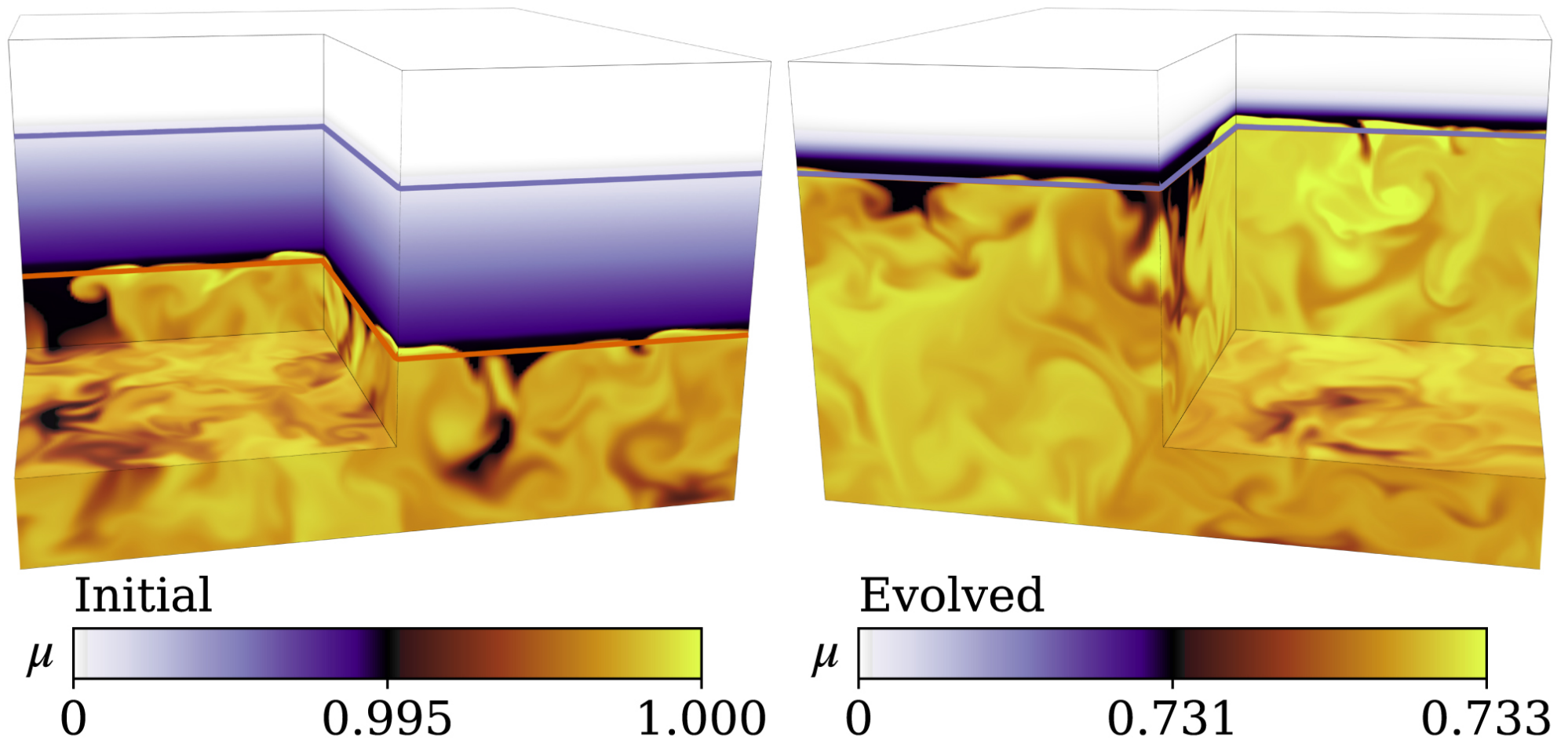
Figure 1. from Evan H. Anders et al 2022 Astrophys. J. Lett. 928 doi:10.3847/2041-8213/ac5cb5 https://dx.doi.org/10.3847/2041-8213/ac5cb5 © 2022. The Author(s). Published by the American Astronomical Society.
