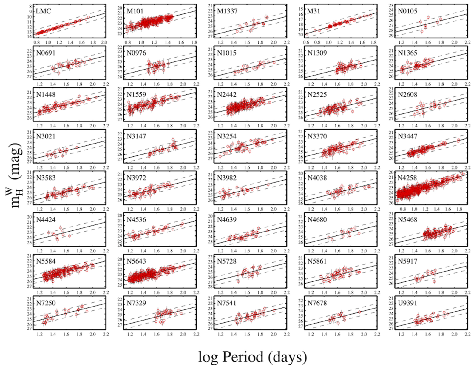
Figure 9. from Adam G. Riess et al 2022 Astrophys. J. Lett. 934 doi:10.3847/2041-8213/ac5c5b https://dx.doi.org/10.3847/2041-8213/ac5c5b © 2022. The Author(s). Published by the American Astronomical Society.
