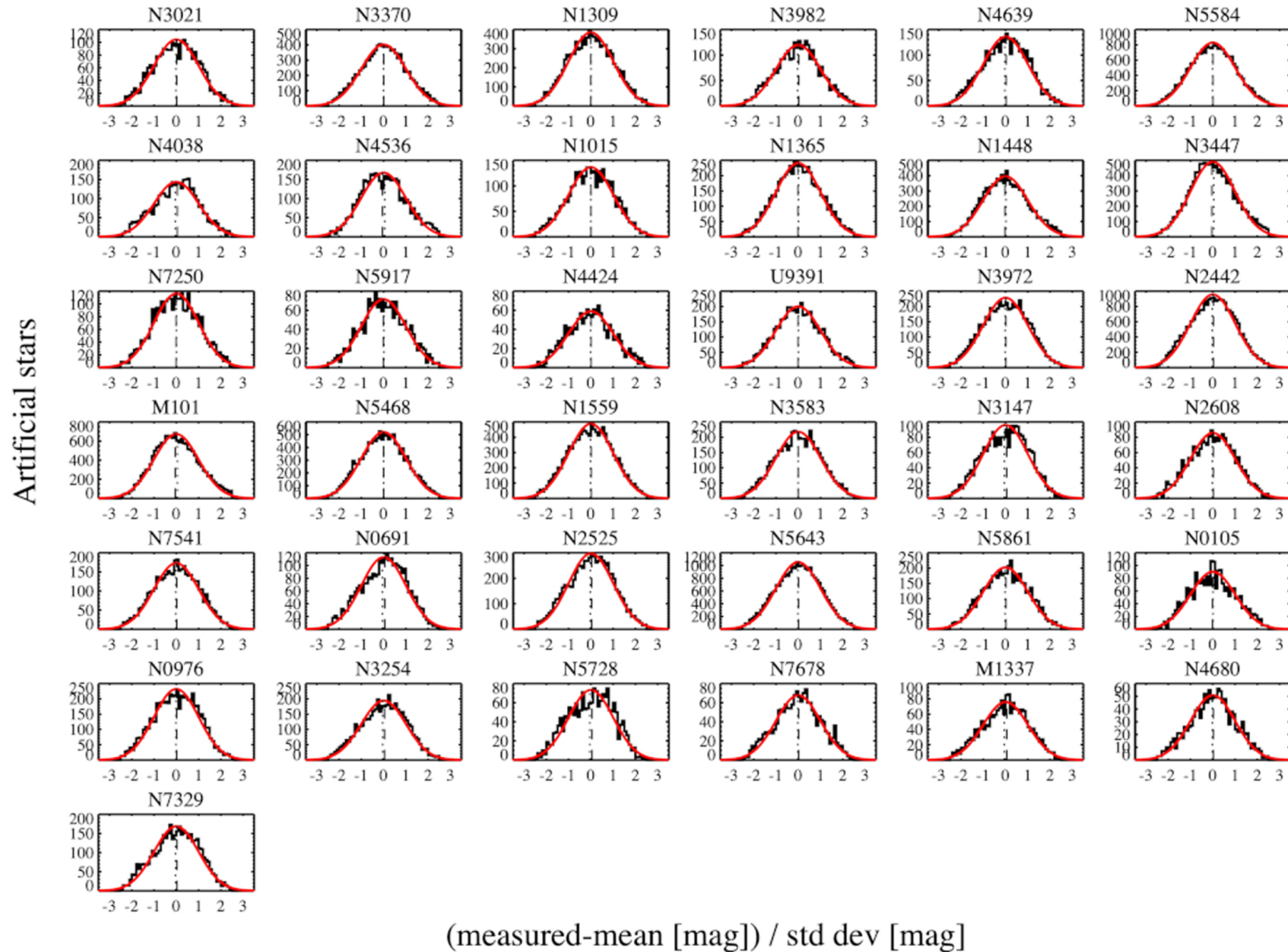
Figure 7. from Adam G. Riess et al 2022 Astrophys. J. Lett. 934 doi:10.3847/2041-8213/ac5c5b https://dx.doi.org/10.3847/2041-8213/ac5c5b © 2022. The Author(s). Published by the American Astronomical Society.
