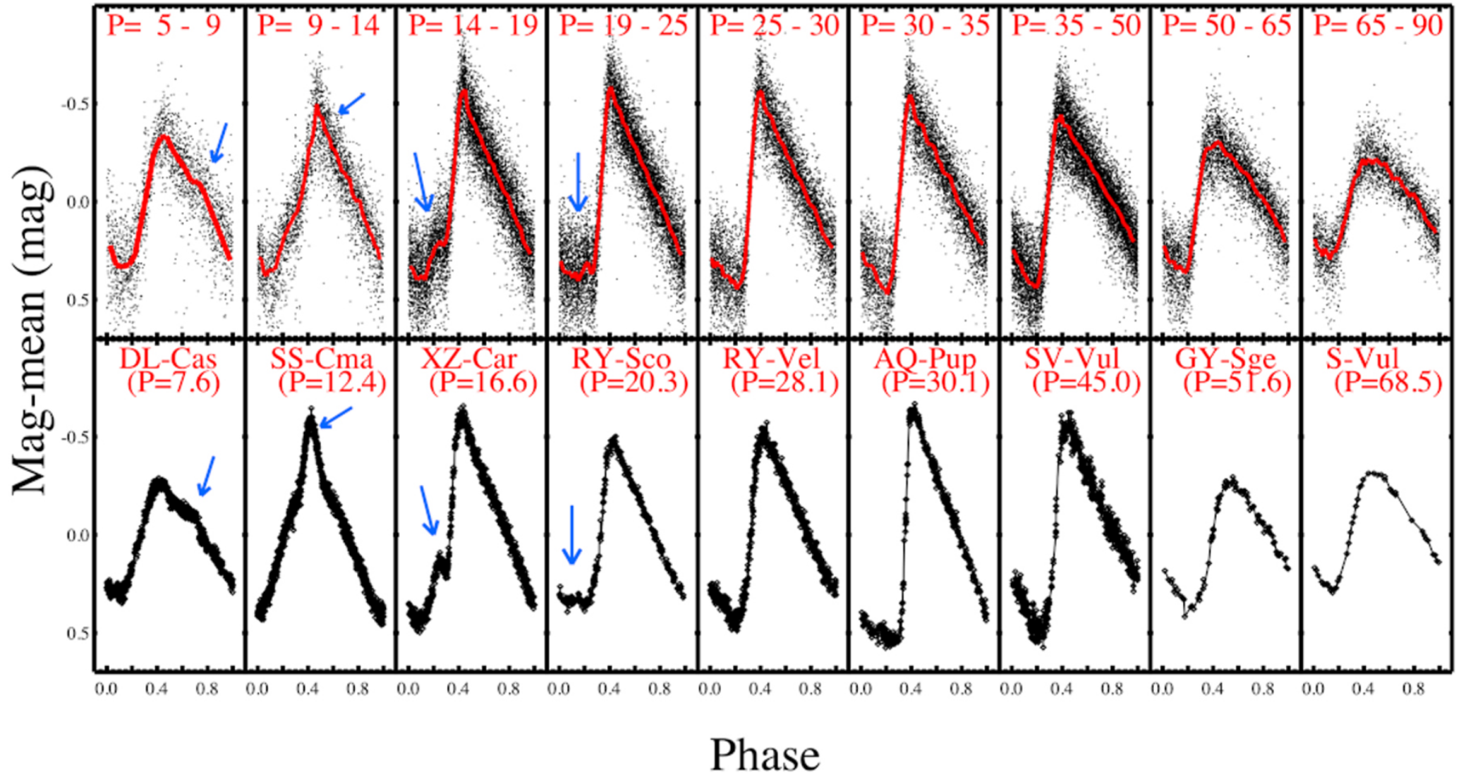
Figure 6. from Adam G. Riess et al 2022 Astrophys. J. Lett. 934 doi:10.3847/2041-8213/ac5c5b https://dx.doi.org/10.3847/2041-8213/ac5c5b © 2022. The Author(s). Published by the American Astronomical Society.
