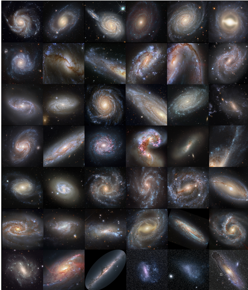
Figure 4. from Adam G. Riess et al 2022 Astrophys. J. Lett. 934 doi:10.3847/2041-8213/ac5c5b https://dx.doi.org/10.3847/2041-8213/ac5c5b © 2022. The Author(s). Published by the American Astronomical Society.
