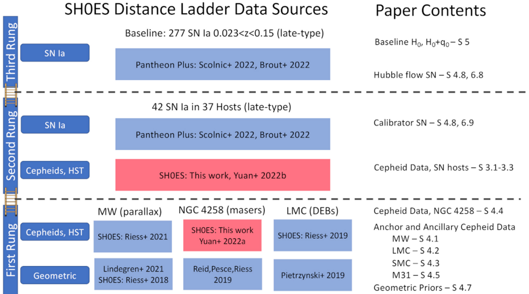
Figure 1. from Adam G. Riess et al 2022 Astrophys. J. Lett. 934 doi:10.3847/2041-8213/ac5c5b https://dx.doi.org/10.3847/2041-8213/ac5c5b © 2022. The Author(s). Published by the American Astronomical Society.
