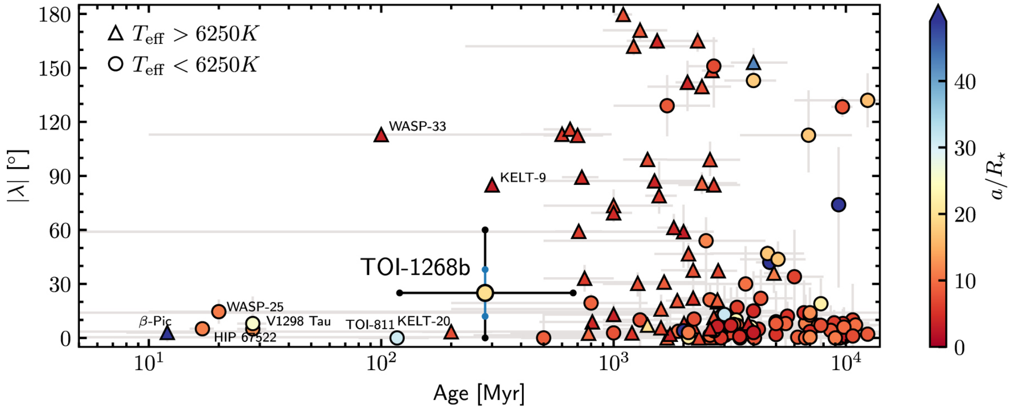
Figure 6. from NEID Rossiter–McLaughlin Measurement of TOI-1268b: A Young Warm Saturn Aligned with Its Cool Host Star null 2022 APJL 926 L7 doi:10.3847/2041-8213/ac4da0 https://dx.doi.org/10.3847/2041-8213/ac4da0 © 2022. The Author(s). Published by the American Astronomical Society.
