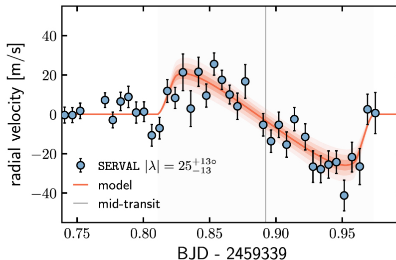
(b) Radial velocities reduced by the SERVAL pipeline
