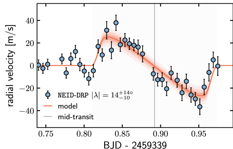
(a) Radial velocities reduced by the NEID-DRP v1.1.2 pipeline
