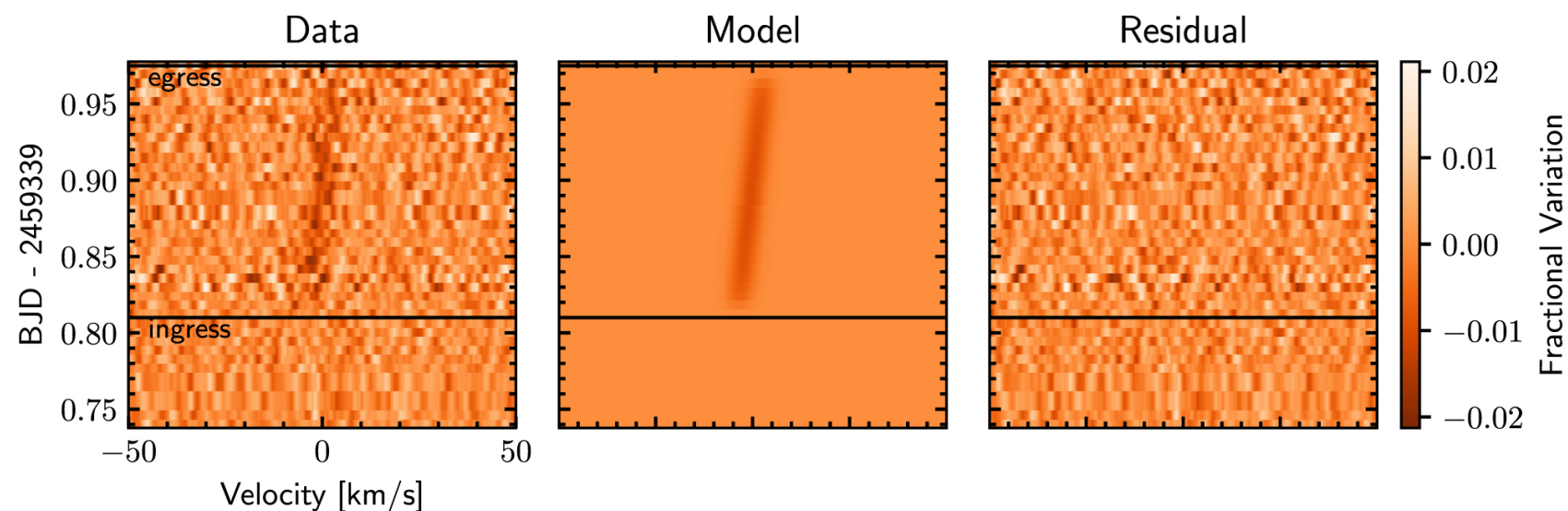
(c) Doppler Tomography signals, from which we infer |\lambda| = 40^{+7}_{-10}
