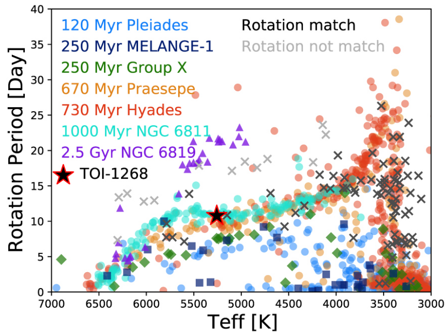
(a) Rotation period vs. effective temperature
