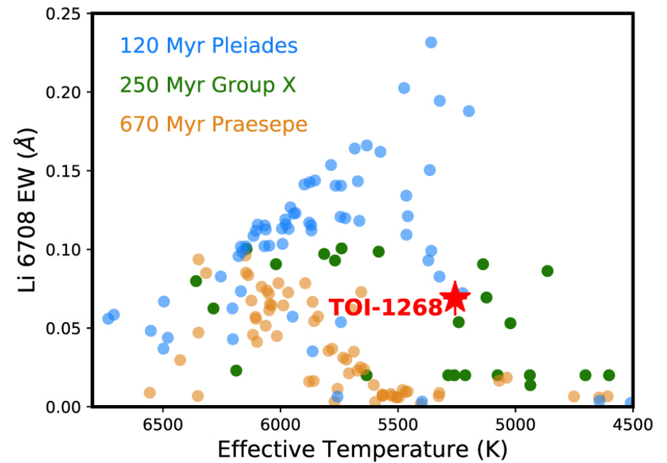
(b) Lithium Equivalent Width (EW) vs. effective temperature
