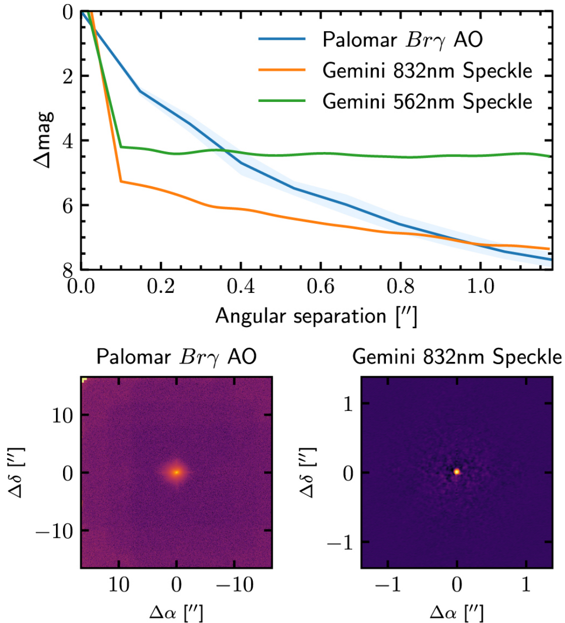
Figure 3. from NEID Rossiter–McLaughlin Measurement of TOI-1268b: A Young Warm Saturn Aligned with Its Cool Host Star null 2022 APJL 926 L7 doi:10.3847/2041-8213/ac4da0 https://dx.doi.org/10.3847/2041-8213/ac4da0 © 2022. The Author(s). Published by the American Astronomical Society.
