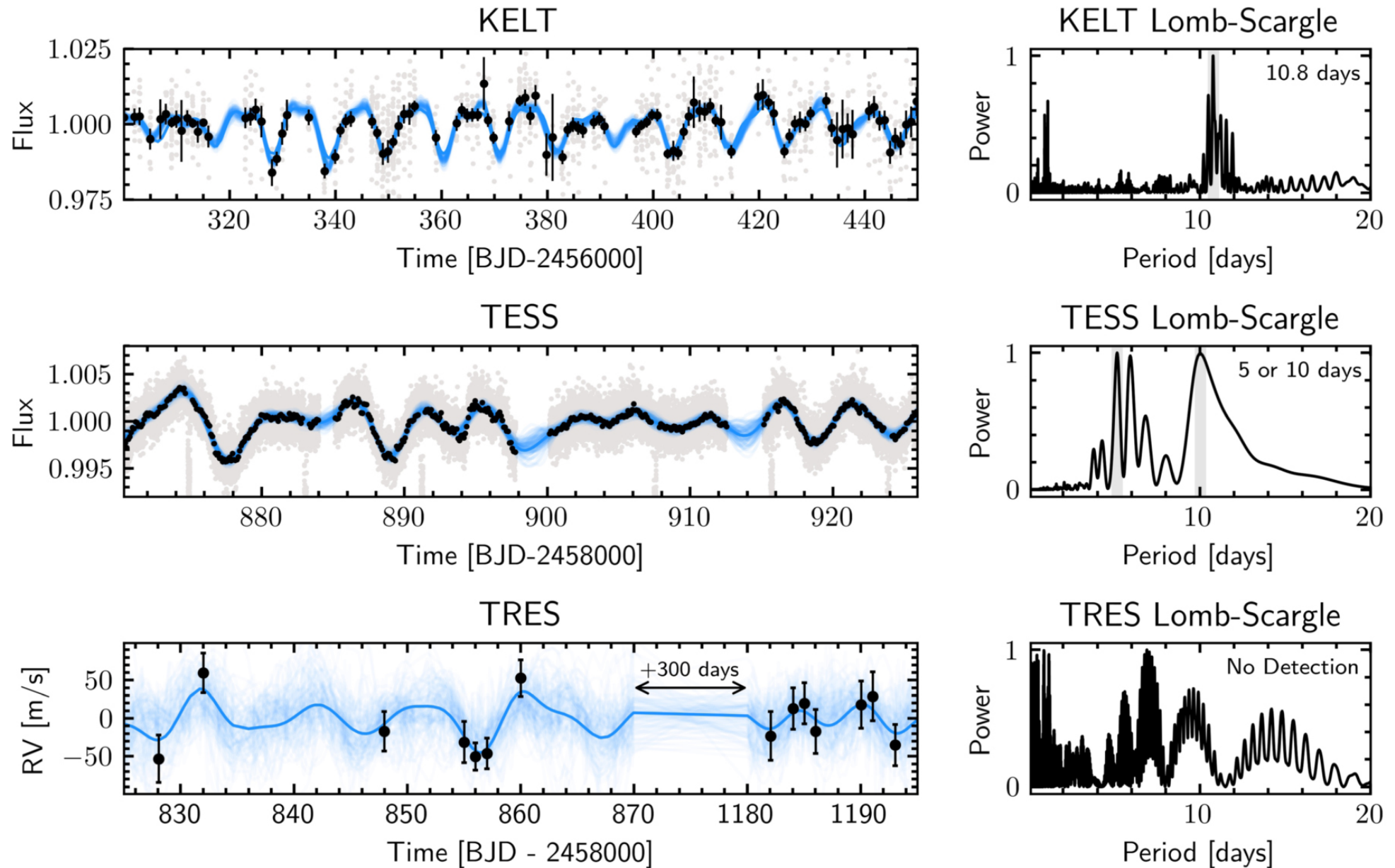
Figure 2. from NEID Rossiter–McLaughlin Measurement of TOI-1268b: A Young Warm Saturn Aligned with Its Cool Host Star null 2022 APJL 926 L7 doi:10.3847/2041-8213/ac4da0 https://dx.doi.org/10.3847/2041-8213/ac4da0 © 2022. The Author(s). Published by the American Astronomical Society.
