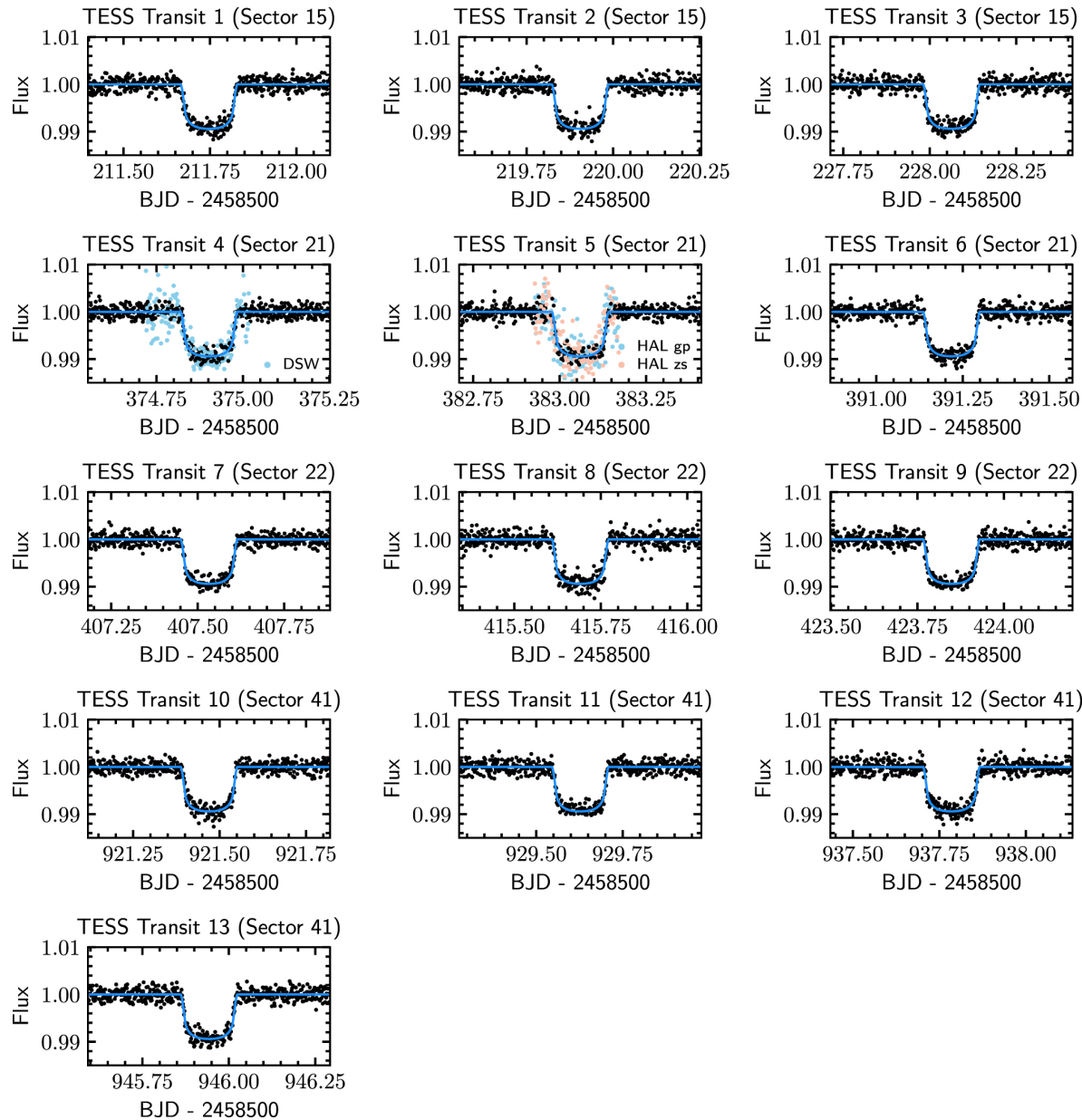
Figure 1. from NEID Rossiter–McLaughlin Measurement of TOI-1268b: A Young Warm Saturn Aligned with Its Cool Host Star null 2022 APJL 926 L7 doi:10.3847/2041-8213/ac4da0 https://dx.doi.org/10.3847/2041-8213/ac4da0
