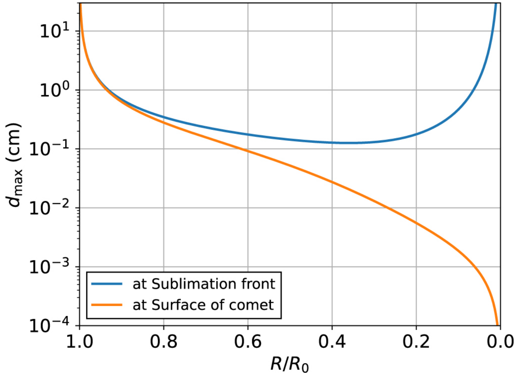
Figure 5. from The Asteroid 162173 Ryugu: a Cometary Origin null 2022 APJL 925 L15 doi:10.3847/2041-8213/ac4bd5 https://dx.doi.org/10.3847/2041-8213/ac4bd5 © 2022. The Author(s). Published by the American Astronomical Society.
