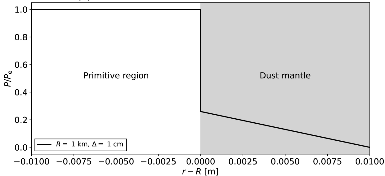
(a) Pressure distribution around sublimation front
