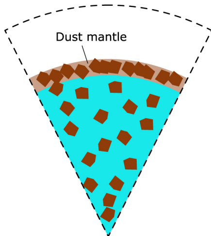
(c) Formation of dust mantle
