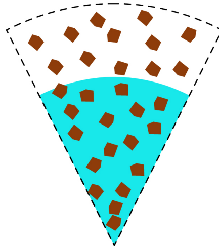
(b) Sublimation of ice
