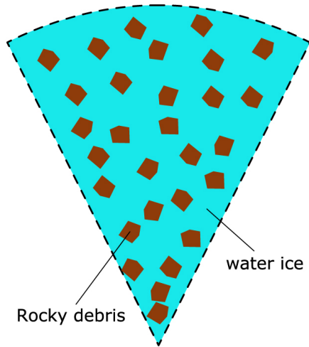
(a) Primitive cometary nucleus
