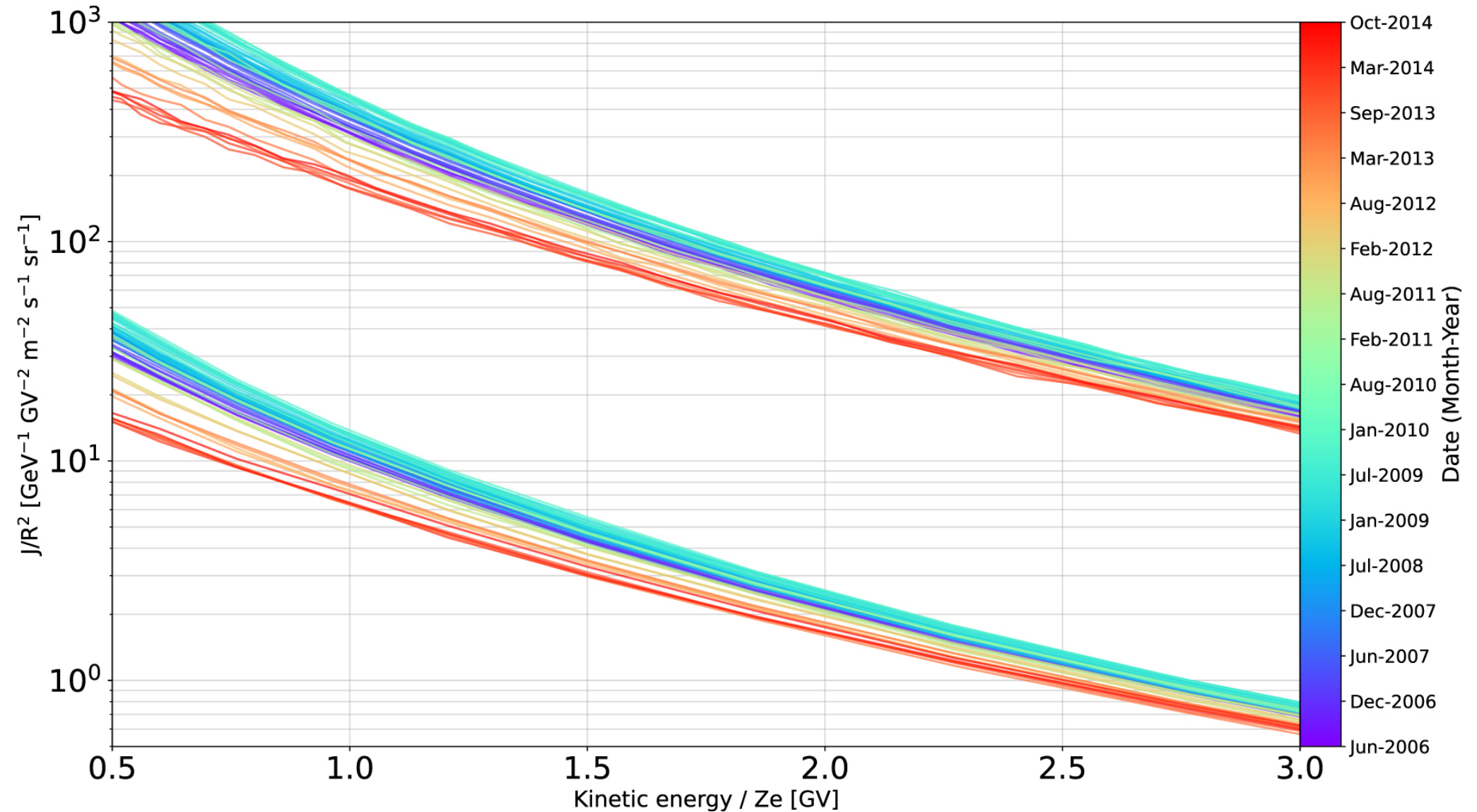
Figure 5. from Helium Fluxes Measured by the PAMELA Experiment from the Minimum to the Maximum Solar Activity for Solar Cycle 24 null 2022 APJL 925 L24 doi:10.3847/2041-8213/ac4787 https://dx.doi.org/10.3847/2041-8213/ac4787 © 2022. The Author(s). Published by the American Astronomical Society.
