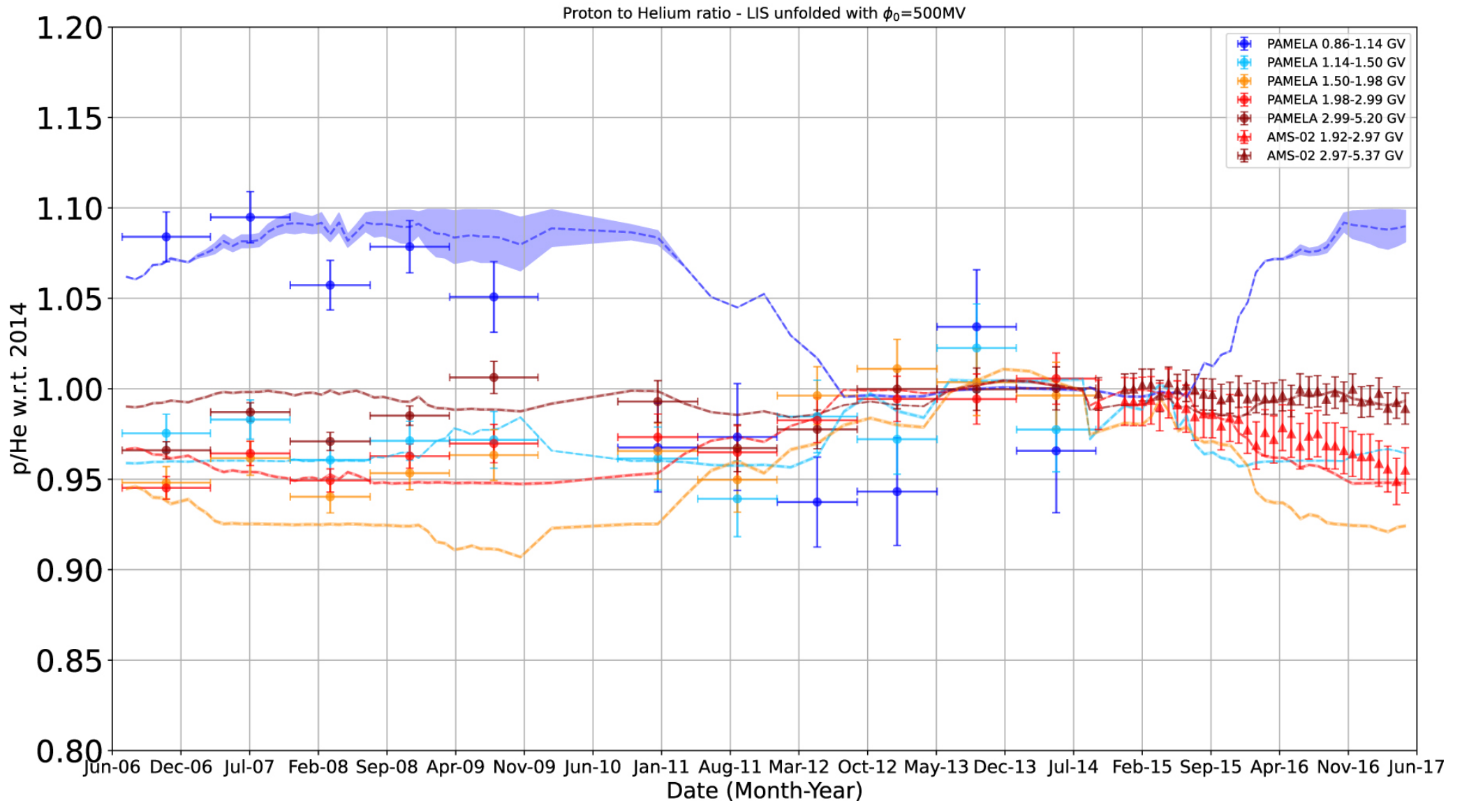
Figure 4. from Helium Fluxes Measured by the PAMELA Experiment from the Minimum to the Maximum Solar Activity for Solar Cycle 24 null 2022 APJL 925 L24 doi:10.3847/2041-8213/ac4787 https://dx.doi.org/10.3847/2041-8213/ac4787 © 2022. The Author(s). Published by the American Astronomical Society.
